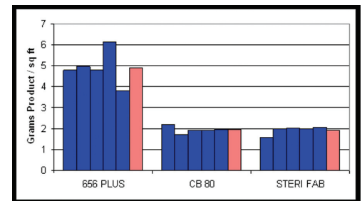
Fig. 13. Application rates, by replicate, of pyrethroid-based contact products.
