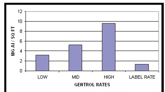
Fig. 9. Mean application rates for Gentrol aerosol.
