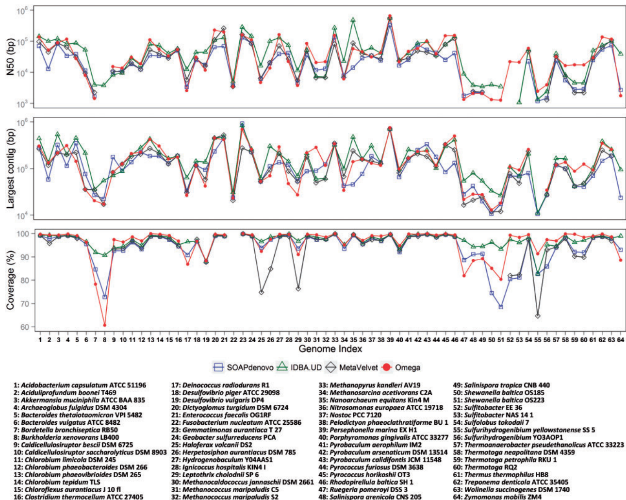
Fig. 2. Scaffold assembly statistics for individual genomes from the HiSeq 100-bp dataset. The x-axis lists the 64 genomes in alphabetic order, and the indices and organism names of the genomes are shown in the legend. The assemblies were provided by SOAPdenovo (blue squares), IDBA-UD (green triangles), MetaVelvet (black diamonds) and Omega (solid red circles). Outliers below the minimum threshold of a performance statistics are not shown
