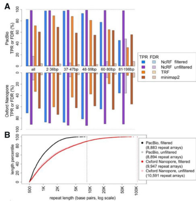
Fig. 1. (A) Performance of NCRF, TRF, and Minimap2 on simulated PacBio (upper panel) and Nanopore (lower panel) reads, binned by motif lengths. Solid bars are TPRs, crosshatched bars are FDRs. All 847 arrays totaled 822 kb, with 197 arrays and 170 kb for lengths 2–36 bp, 156/158 kb for 37–47 bp, 158/173 kb for 48–59 bp, 172/162 kb for 60–80 bp and 164/160 kb for 81–198 bp. (B) Observed lengths of (AATGG) n arrays (with and without consensus filtering) in PacBio and Nanopore reads. Reads were subsampled to a similar length distribution of 16.5 Gb (Supplementary Note S5). Filtered and unfiltered results for PacBio are very similar
