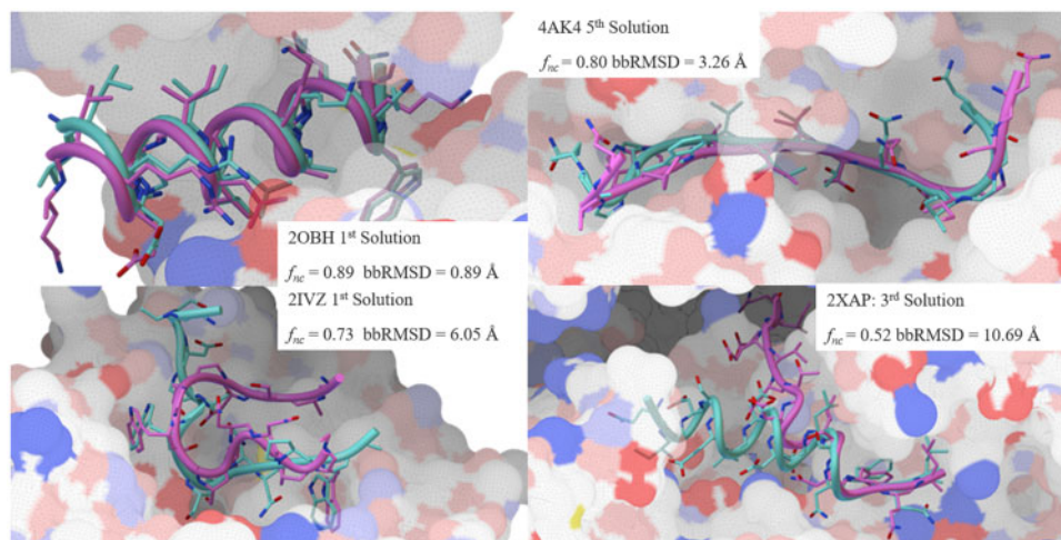
Fig. 4. Comparison of selected docked poses (cyan) and experimentally determined structures (magenta). The receptor surface is provided for context and colored using a polarity scheme developed by Dr. D. Goodsell. These Figures are generated using PMV 1.5.7 (Sanner, 1999) and MSMS (Sanner et al. , 1996) (Color version of this figure is available at Bioinformatics online.)
