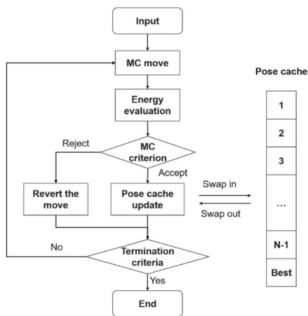
Fig. 2. Flow chart of AutoDock CrankPep Monte Carlo procedure
