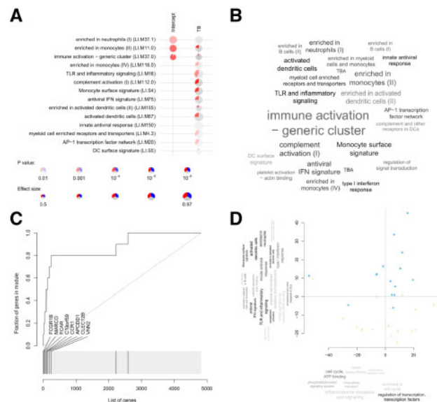
Fig. 1. Examples of tmod package graphical illustrations of enrichment results. (A) A panel plot which allows presentation of large number of comparisons; (B) a tag cloud for enriched GS; (C) evidence plot for a selected GS, where the AUC corresponds to effect size; (D) principle component analysis combined with enrichment allows to functionally annotate the components
