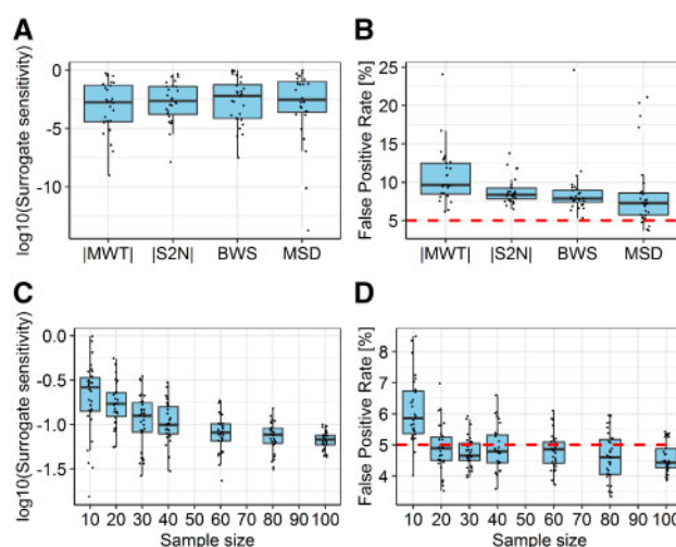
Fig. 3. Comparison of the impact of different gene ranking metric (top row) and sample sizes (bottom row) on the surrogate sensitivity (lower is better) and FPR (closer to 5% is better) for the CERNO algorithm. Panels (A) and (B) represent impact of different ranking metrics in terms of surrogate sensitivity and FPR at various sample size, respectively. Panels C and D represent impact of sample size to surrogate sensitivity and FPR for MSD metric only. Red line on panels (B) and (D) represents the expected FPR level
