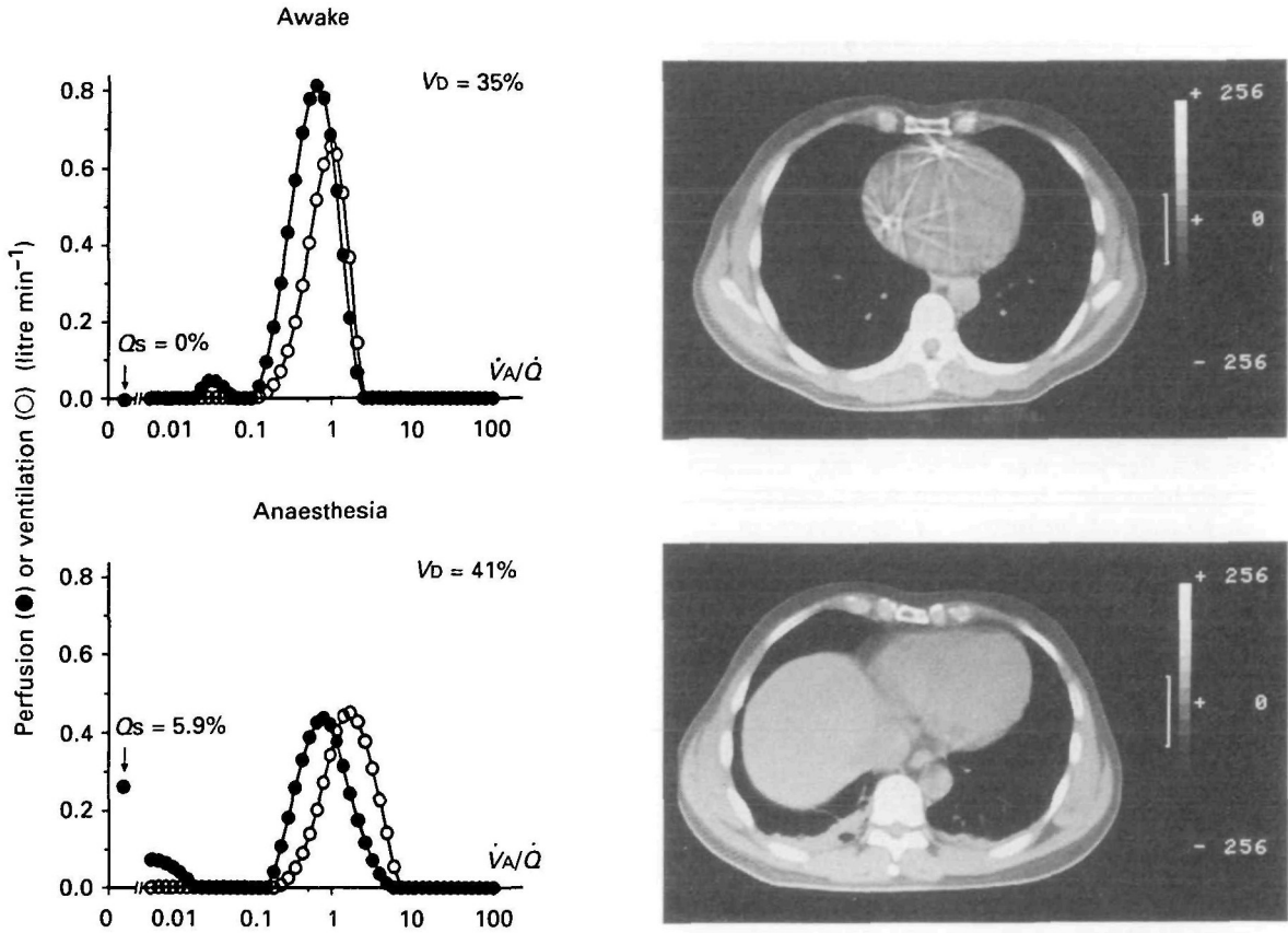
FIG. 1. Normal pattern of gas exchange and CT scans (caudal level) awake and during anaesthesia. Ventilation-perfusion distribution to the left; CT scan of the chest to the right. Note the increase in shunt, log SD \dot{V}_A/\dot{Q} (widened \dot{V}_A/\dot{Q} mode), and low \dot{V}_A/\dot{Q} , in addition to the atelectatic areas in the dorsal part of the CT scan during anaesthesia. The large white area in the middle of the right hemithorax (lower CT scan) is the diaphragm that has moved cranially during anaesthesia.
