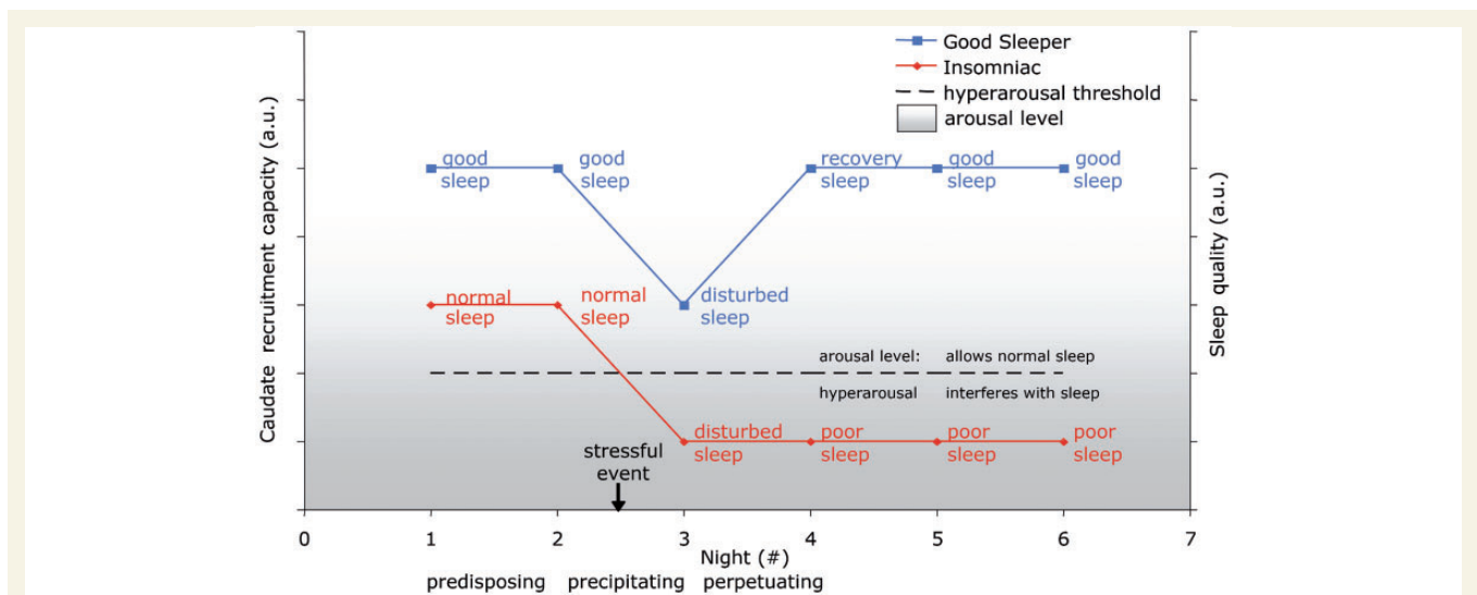
Figure 4 Limitations in the capacity for caudate recruitment may both predispose to, and perpetuate, hyper-arousal and insomnia. Patients with insomnia have a constitutionally lower capacity to recruit the head of the caudate, predisposing them to increased arousal. When an external factor (sleep manipulation in the laboratory, stress in real life) disrupts sleep, the capacity to recruit the head of the caudate is further reduced. In people without the aforementioned predisposition this will not bring their arousal level into the realm of hyper-arousal, which consequently normalizes as soon as a precipitating factor is no longer present. In people with the predisposition, a further reduction of their already limited caudate recruitment capacity, elicited by a night of disrupted sleep, could bring it to a level so low that it can no longer sufficiently inhibit autonomic and CNS responses to sensory input. The resulting hyper-aroused state of behavioural restlessness, hyper-responsivity and elevated autonomic and cortical excitability is in itself sufficient to interfere with sleep, thus perpetuating both the limited caudate recruitment capacity and disturbed sleep. a.u. = arbitrary units.
