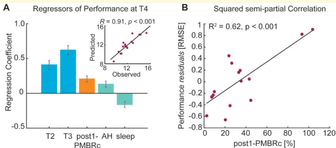
Figure 5 Prediction of motor performance at T4. Regression analysis provided statistically significant performance prediction (A) as quantified by the correlation between actual and predicted motor performance in stroke patients (inset figure), with significance determined by permutation-testing. The model consisted of five significant predictors accounting for 82% of variance in performance 24 h after training (T4). Patients' performance during training, post-training movement-related beta activity, affected hand and sleep quantity were related to performance at T4. Z-scored regression coefficients ( \beta ) quantify the influence of each significant predictor upon performance level at T4. Error bars represent standard error of the mean. (B) Importantly, post hoc squared semi-partial correlation confirmed that movement-related beta activity immediately after training was positively related to performance at T4, indicating that smaller magnitude of contralateral (ipsilesional) PMBR is associated with better future performance.
