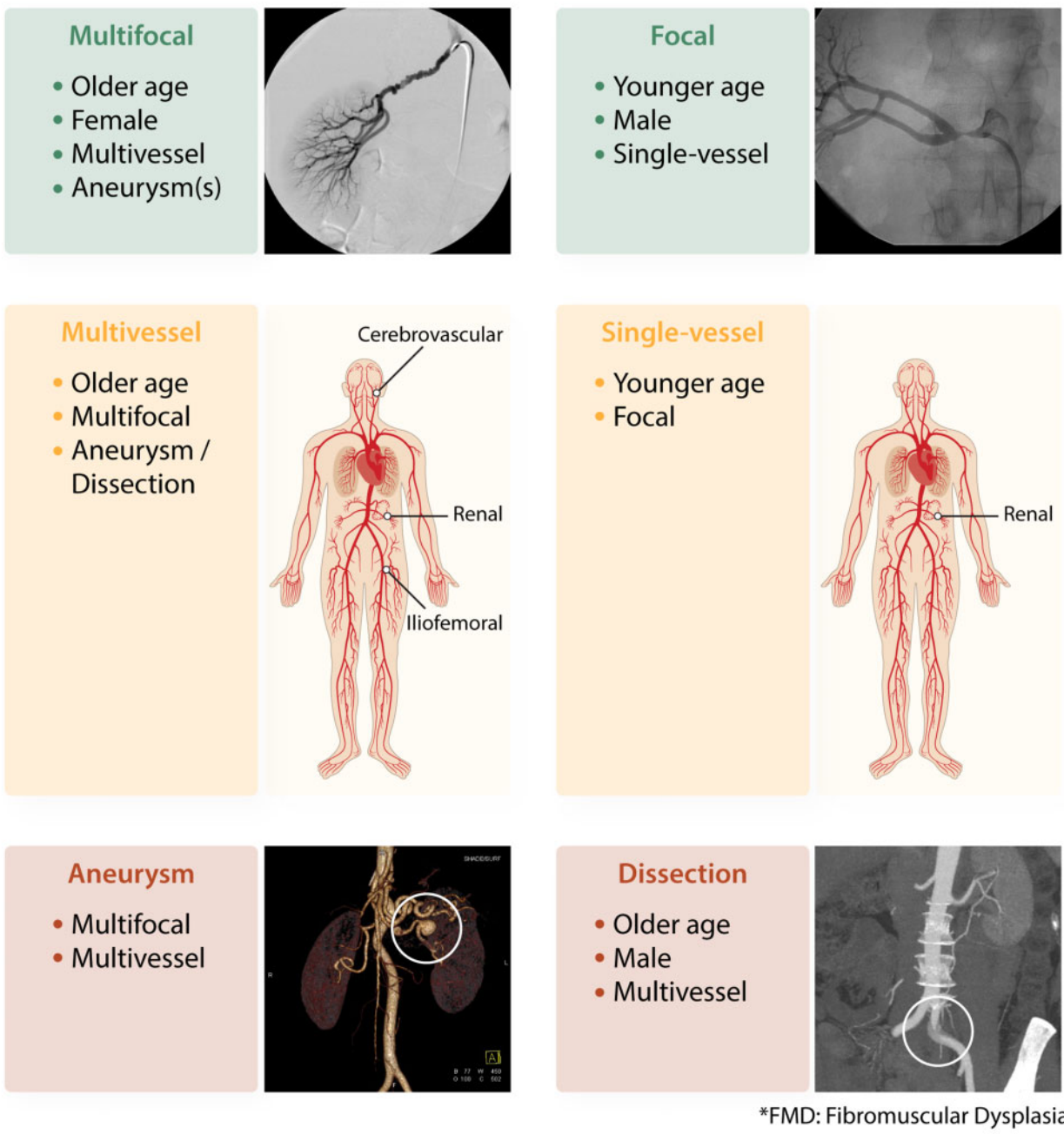
Figure 2 Typical features of patients with multifocal/focal FMD, multivessel/single-vessel FMD, and FMD with aneurysm(s) or dissection(s) based on findings of the European/International FMD Registry. FMD, fibromuscular dysplasia.
