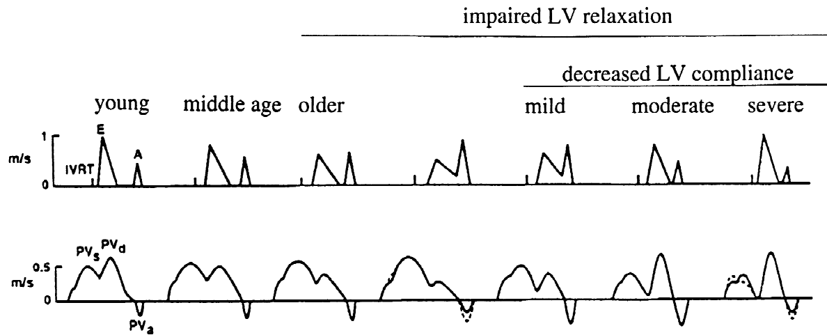
Fig. 2. Schematic representation of transmitral and pulmonary venous flow pattern according to Appelton and Hatle [21]. With increasing age the E/A ratio decreases. In elderly patients the ratio is less than 1 ('impaired relaxation' pattern) and the pulmonary venous flow shows a decrease in diastolic flow (PVd). In subjects with impaired LV relaxation (e.g. myocardial hypertrophy, ischemia) the filling pattern shows a further decrease in the E-wave, whereas with a decrease in LV compliance the filling pattern changes towards normal ('pseudo-normalization') and even shows enhanced early diastolic filling with an E/A ratio >2 ('restrictive filling' pattern). With the progressive decrease in LV compliance pulmonary venous flow shows a diminution of systolic flow with an enhanced early diastolic flow and a reversal of atrial flow.
