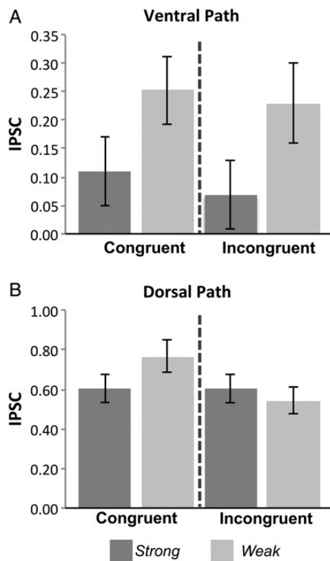
Figure 4. The ventral and dorsal pathways are involved in separable control processes. Activation in regions defined a priori along the ventral path (top) track the modulation of Strength rather than Congruency or the interaction of both factors. Importantly, significantly greater activation is observed for Weak than Strong within the Incongruent condition ( P < 0.05 ), a pattern inconsistent with a response selection effect. In contrast, activation in regions defined a priori along the fronto-parietal “dorsal path” (bottom) reliably track the interaction of Strength and Congruency, implicating this pathway in postretrieval selection rather than memory access. Error bars depict within-subject standard error.
