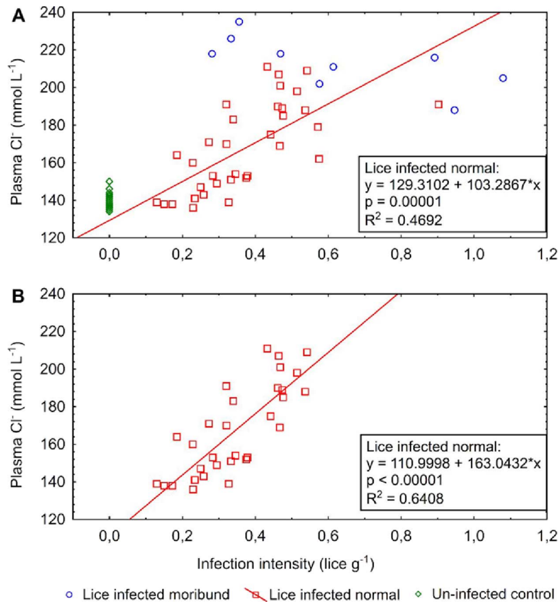
Figure 1: Simple regressions between infection intensity (lice g -1 ) and plasma Cl - (mmol L -1 ). (A) Trend line, P and R 2 values are based on data from the lice infected normal group. Data from lice infected moribund fish and the uninfected control group are included for comparison. (B) Data from lice infected normal fish with infection intensity < 0.55 lice g -1 (mean infection intensity in dead fish).
