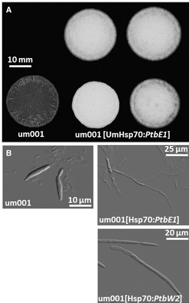
Figure 7 Single Pt b alleles are functional and interact with the Um b -regulated pathway controlling the switch from yeast-like to filamentous growth. In this representative example, Pt bE1 or Pt bW2 cDNA was expressed from the strong Um Hsp70 promoter and terminator elements. Four independent haploid Um integrative transformants displayed filamentous growth shown as aerial hypha when spotted on charcoal medium (Fuzz + colony phenotype; A) and by light microscopy (B). cDNA, complementary DNA; Pt , Puccinia triticina ; Um , U. maydis .
