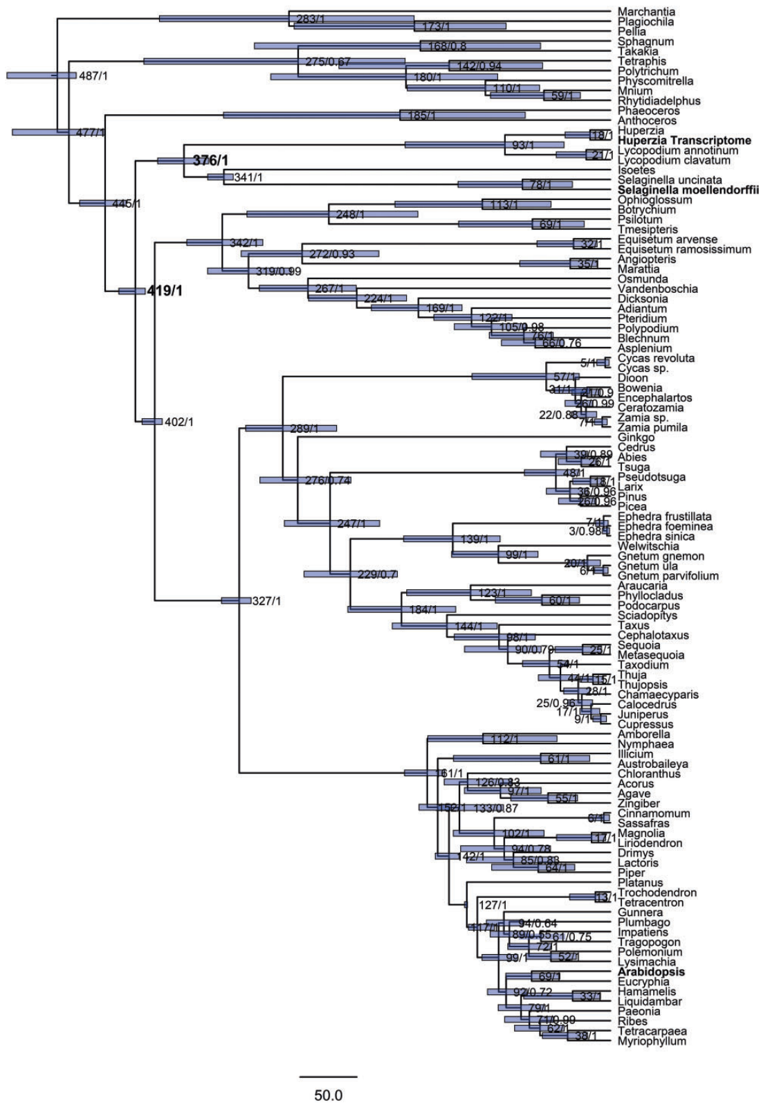
Fig. 3. —Dated phylogeny inferred from analysis of three chloroplast genes ( atpB , rbL , and rps4 ), using a Bayesian framework and a relaxed molecular clock. Values represent node ages (median heights), followed by posterior probabilities of clades. Blue bars illustrate the node height 95% HPD intervals. The most recent common ancestor of Huperzia and Selaginella is estimated to have existed about 376 Ma, and that of Huperzia and Arabidopsis about 419 Ma. Accession numbers of all sequences used in the phylogeny are given in supplementary table S1, Supplementary Material online.
