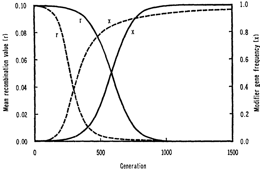
FIGURE 1.—Changes in the modifier gene frequency and the mean recombination value due to natural selection; haploid system. Fitness, W_1 = 1, W_2 = W_3 = 0.5, W_4 = 1 . The solid line refers to the case of r_0 = 0.1, r_1 = 0.05, r_2 = 0.0 and the broken line to the case of r_0 = 0.1, r_1 = r_2 = 0.0 .
