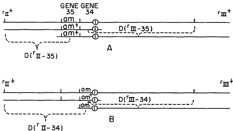
FIGURE 4.—The arrangement of genes 35 (A) or 34 (B) on fragments, which appears necessary for these genes to express their function.—⊖ indicates the position of the necessary starting region. The two lower solid lines indicate the right hand and left hand extensions of fragments which are necessary for expression of genes 35 or 34. The broken lines reflect the apparent distances which result from these restrictions.
