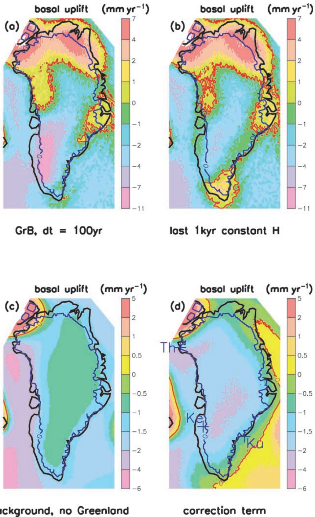
Figure 14. Rate of basal uplift over last 100 yr for (a) model GrB and (b) for model GrB but with ice field frozen for last 1000 yr. Also shown are (c) the contribution to the rate of present day basal uplift from the non-Greenland components of ICE-4G and (d) the correction term for computing full rate of basal uplift that includes both ICE-4G non-Greenland and non-eustatic ocean load components (refer to text for details).
