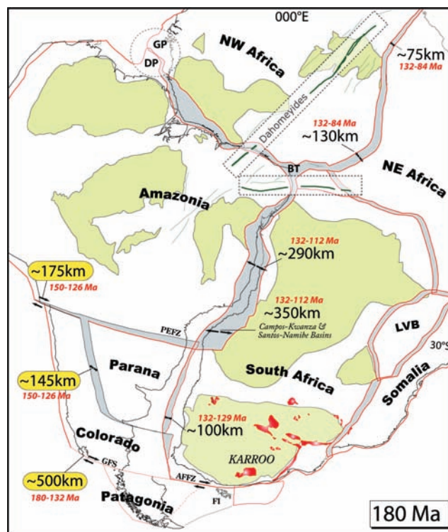
Figure 10. A pre-drift reconstruction of the South Atlantic realm at ~180 Ma. GP, Guinea Plateau; DP, Demara Plateau; BT, Benue Trough; PEFZ, Paraná-Etendeka Fracture Zone; AFFZ, Agulhas-Falkland Fracture Zone; GFS, Gastre Faults System; FI, Falkland Islands; MEB, Maurice Ewing Basin; LVB, Lake Victoria Block. Ages in red denote the total length of pre-drift extension/strike-slip.
