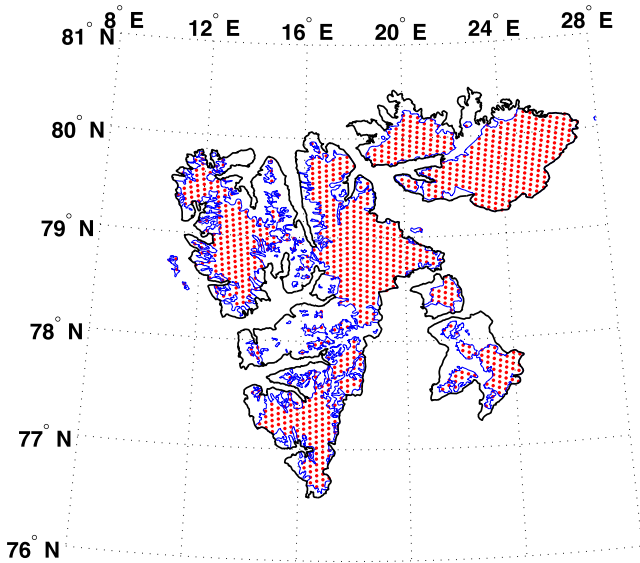
Figure 6. Discretization of the ice-covered area, bounded by the blue line, during the LIA by means of surface disc loads. Red dots mark the centers of discs with an area of 32 \text{ km}^2 each.
