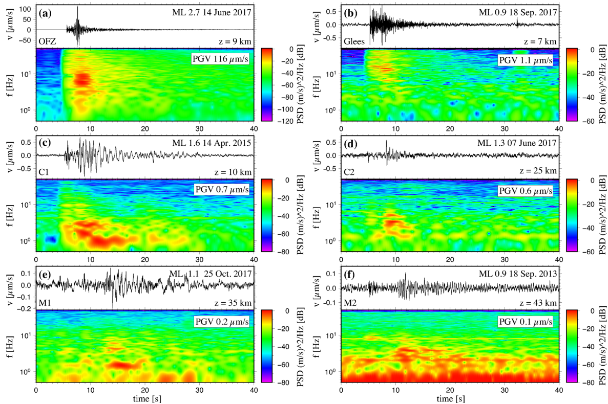
Figure 4. Waveform and spectrogram plots of exemplary earthquakes of each cluster. Both upper panels show high frequent brittle earthquakes of the OFZ (a) and the southern Glees 1 cluster (b), all following panels (c–f) show DLF earthquakes at various depths. The vertical component of station Ochtendung (OCHT), about 10 km SSE of Laacher See Volcano is displayed, except for the September 2013 event (f), where the station Ahrweiler (AHRW) is chosen, as OCHT was not yet installed by that time.
