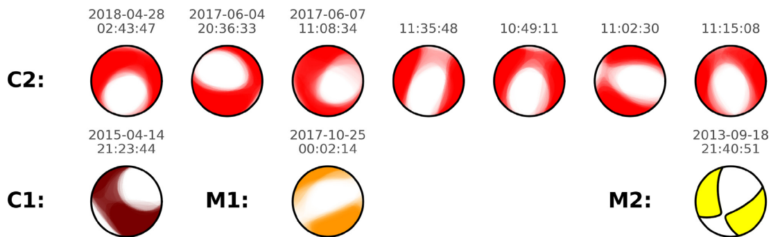
Figure 7. Moment tensor solutions of DLF earthquakes from Table 2. The fuzzy moment tensor plots show the P -wave radiation patterns (lower hemispheric projections), where intensities of colours give the normalized amplitude radiation from the ensemble solutions of the first dominant cluster. For the M2 cluster (2013), the best-fitting solution based on amplitude ratios is shown. Colours represent different cluster depths as defined in Fig. 1. Events can be identified by day of occurrence and hours (Table 2).
