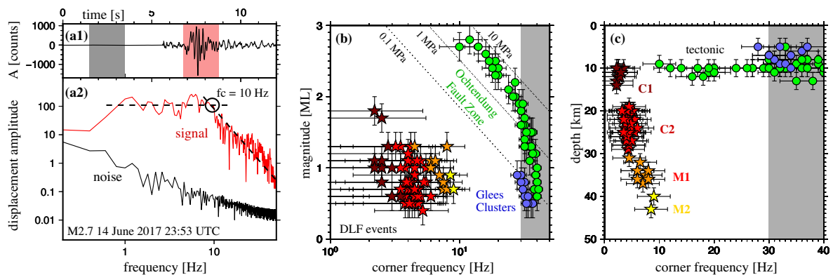
Figure 5. Corner frequencies f_c with respect to magnitude M_L and depth z . Symbols and colors are chosen similar to Fig. 1. Panel (a) gives an example for displacement waveforms and corresponding power spectra of signal (red) and noise (grey/black) of the M_L 2.7 earthquake on the Ochtendung Fault Zone on 2017 June 14. The corner frequency in this example is 10 \pm 3 Hz. Panel (b) shows M_L with respect to f_c . Dotted lines represent the stress drop, the grey box marks frequencies above 30 Hz that were excluded due to anti-alias filtering below f_{Ny} . Panel (c) shows z versus f_c , grey box as in panel (b).
