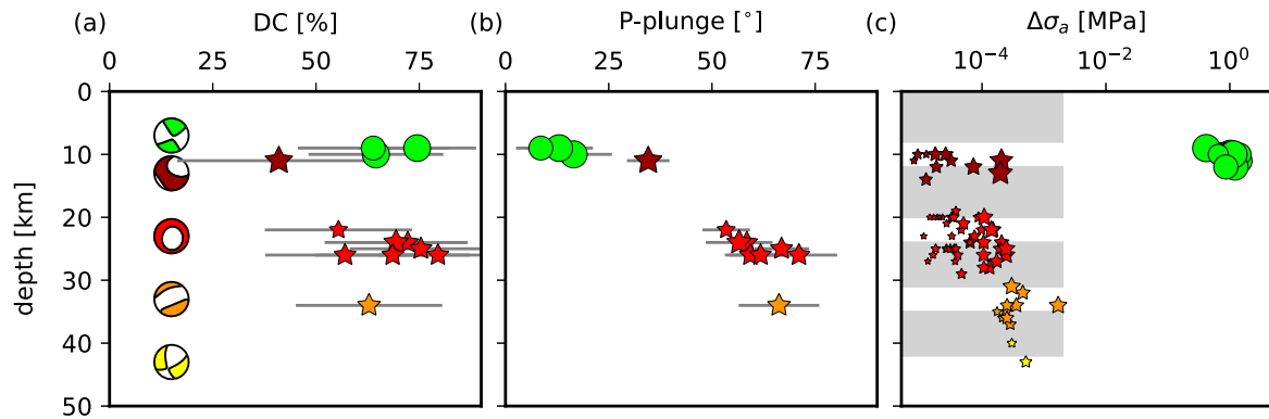
Figure 8. Source parameters from moment tensor analysis. (a) Double-couple components (DC) are plotted together with the P -wave radiation pattern of the representative deviatoric moment tensors (see Fig. 1 for colour scale). For C2 the average moment tensor is plotted. (b) P -axes plunge angle for the different clusters as a function of depth. (c) Apparent stress drop as a function of depth. The stress drop is estimated from the kinematic, self-similar, circular rupture model of Sato & Hirasawa (1973) and our measured corner frequency f_c from \Delta\sigma_a = (7\pi / 16) \cdot (1 / 0.8v_s)^3 M_0 f_c^3 , where a shear wave velocity of v_s \approx 3500 \text{ m s}^{-1} has been assumed. The grey bars show depth ranges of magma storages as postulated by Schmincke (2007).
