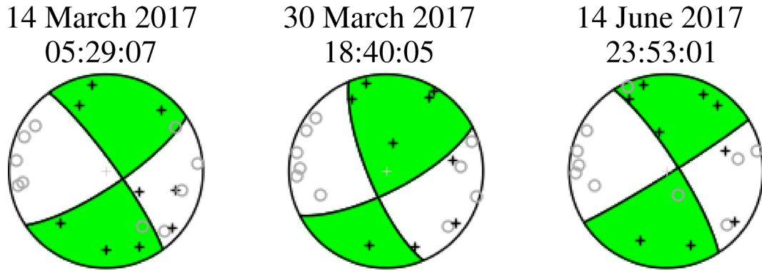
Figure 6. Moment tensor solutions of tectonic earthquakes ( M_L > 2.3 ) on the Ochtendung Fault Zone from 2017 (see red circles in Fig. 1). Best double-couple lower hemispheric projections (Lambert equal area) are plotted together with polarities of P -wave first motions (black crosses positive, white circles negative). Ray piercing points have been calculated using a ray tracer and the CRUST 2.0 model of the Eifel region (Bassin et al. 2000).
