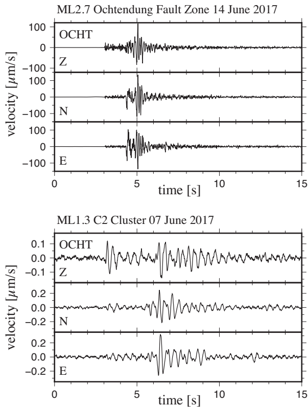
Figure 2. Waveform examples of a tectonic M_L 2.7 earthquake on the Ochtendung Fault Zone (upper panel) and a M_L 1.3 DLF event in the C2 cluster (lower panel). Shown data are from the seismic station Ochtendung (OCHT) southeast of LSV (Fig. 1), time windows are of equal length for frequency comparison.
