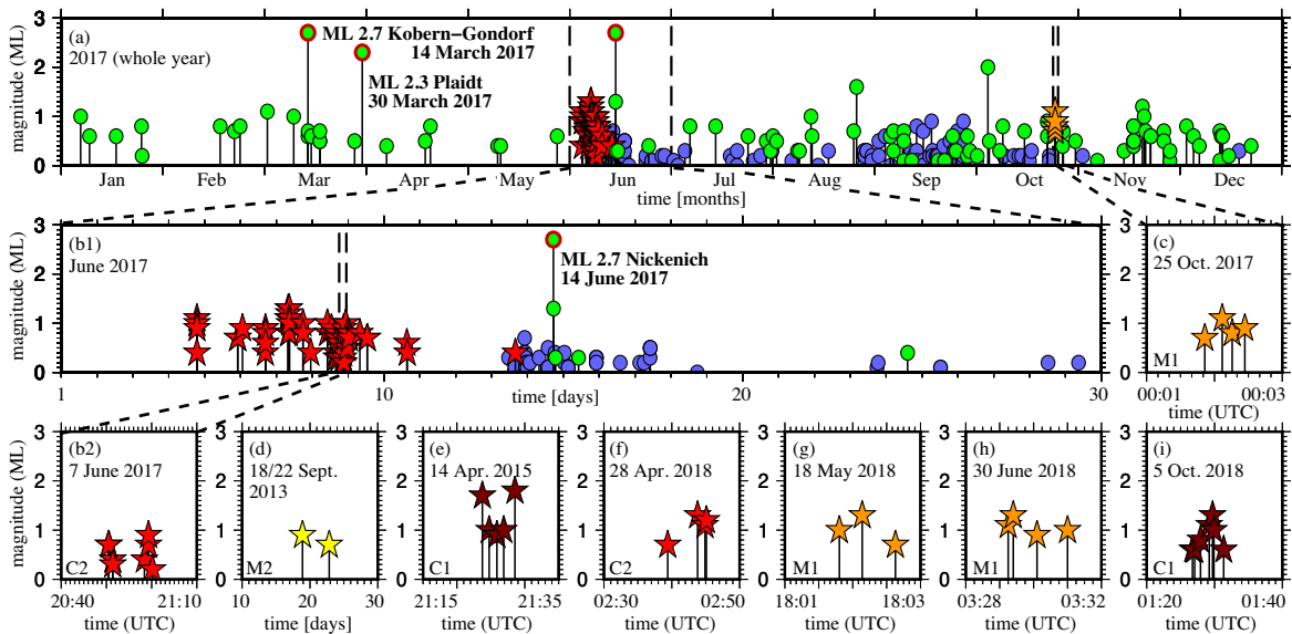
Figure 3. Temporal distribution of earthquake clusters. Colours and symbols are similar to Fig. 1. (a) for the whole year 2017, (b1) for June 2017, (b2) two short pulses within 30 min on 2017 June 7, (c) four events within 36 s on 2017 October 25, (d) two single events on 2013 September 18 and 22, (e) five events within 6 min on 2015 April 14, (f) single event followed by a pulse of three events on 2018 April 28, (g) three events within 50 s on 2018 May 18, (h) four events within 2 min on 2018 June 30 and (i) six events within 7 min on 2018 October 5.
