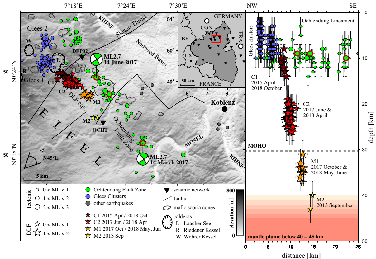
Figure 1. Topographic map of the East Eifel Volcanic Field including faults, calderas and scoria cones. Brittle earthquakes are marked as dots, DLF events as stars. Seismic stations are indicated as inverse triangles. Red circles mark the three largest tectonic earthquakes ( M_L > 2.3 ) in 2017 for which moment tensor solutions are discussed in this study, beach balls are given for the two largest events ( M_L 2.7 ). The city of Koblenz is marked with a black dot. The small overview map outlines the target region as a red box, the state of Rhineland-Palatinate is highlighted in dark grey. LX stands for Luxemburg and BE for Belgium, white dots give the cities of Cologne (CGN) and Frankfurt am Main (FRA). A depth section of all earthquakes is given in the right-hand panel, seen in direction to N45^\circ E . Error bars indicate location uncertainties.
