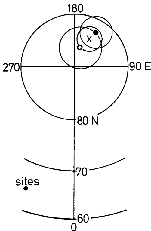
FIG. 4. Means of ( N+R ) lavas (X), R lavas (O) and N lavas (●), with anomalous lavas excluded from the calculations. The 95 per cent circles of confidence are drawn in.
