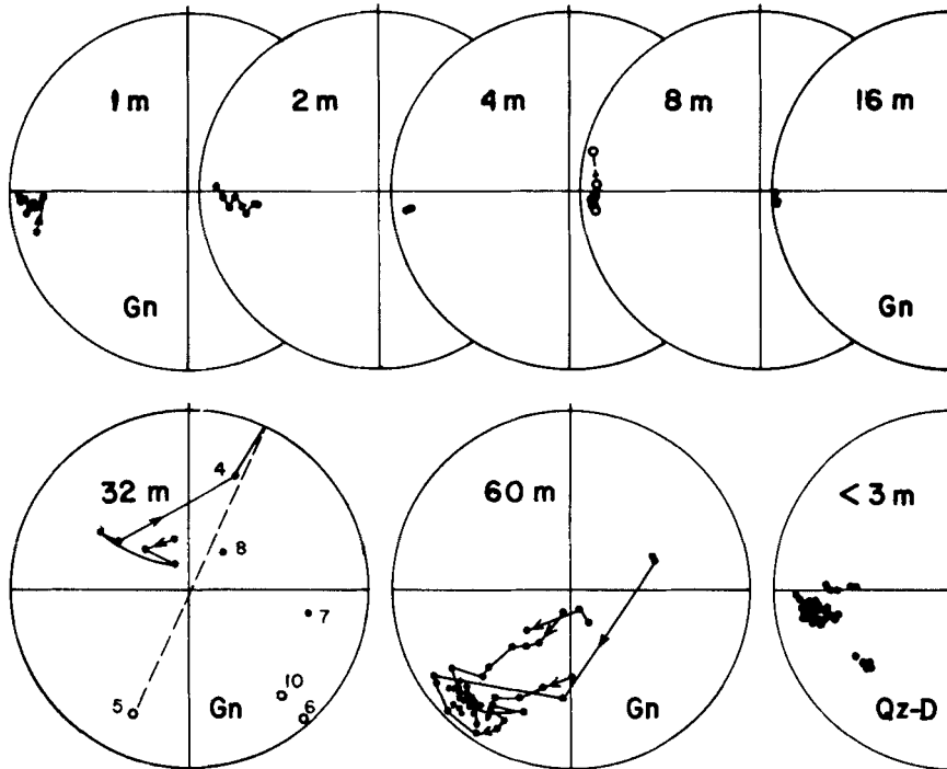
Figure 6. AF demagnetizations (0–100 mT) of gneiss specimens at the distance from the dyke margin as indicated in metres ( cf. Fig. 5). At 60 m distance ( = 2.6 \times dyke width) no resetting is discernable, at 32 m ( = 1.4 \times dyke width) a very scattered directional picture is seen, and at 16 m or less (less than 0.7 \times dyke width) a total resetting by the heating from the dyke is evident in the gneiss (stereographic projection).
