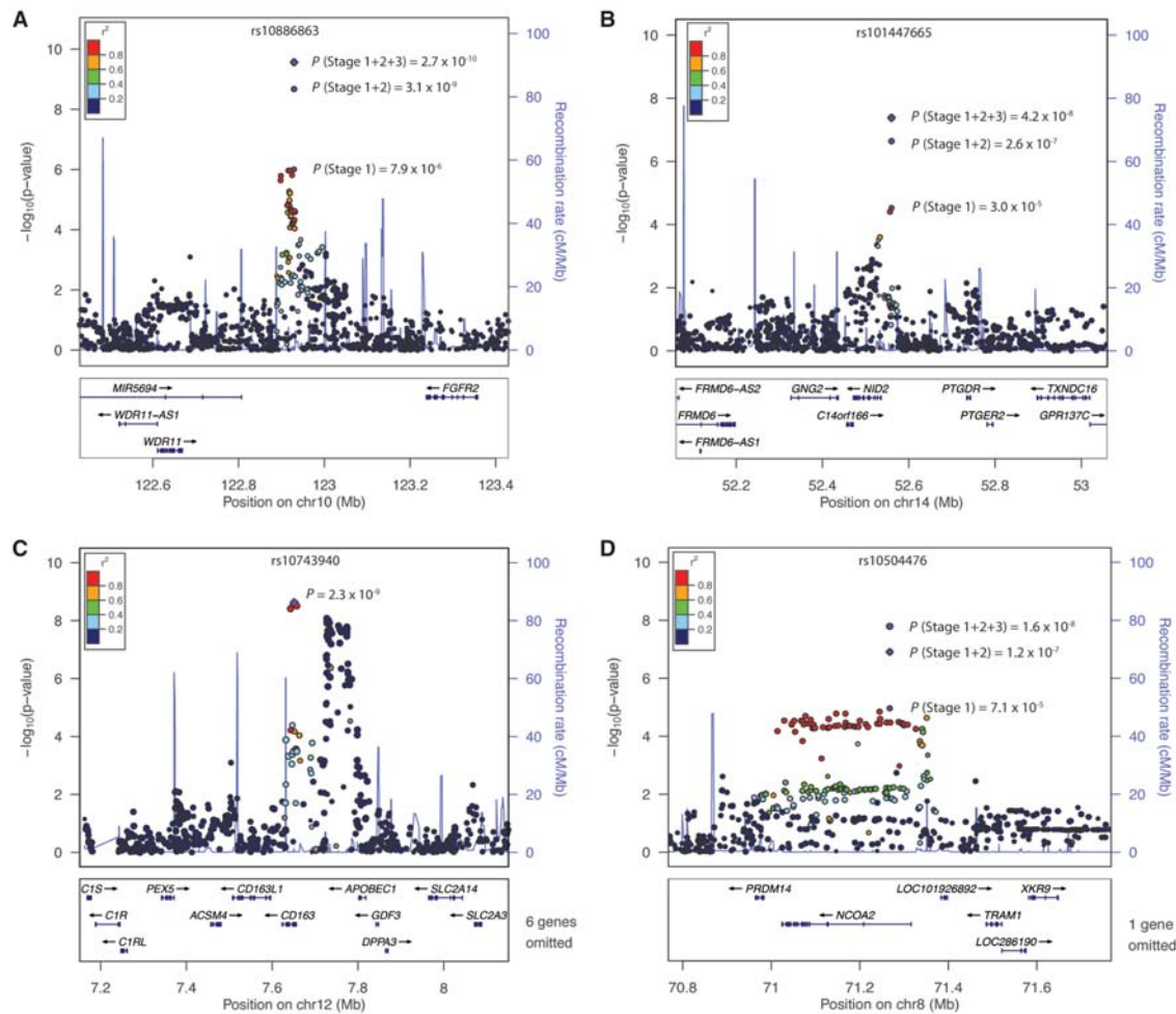
Figure 1. Regional association plots of the four loci identified from East Asian meta-analysis. (A) WDR11-FGFR2, (B) NID2-PTDGR, (C) CD163-APOBEC1, (D) NCOA2. -\log_{10} ( P -values) are plotted against the hg19 genomic coordinates at each locus. The purple circle represents the lead variant, which exhibited the strongest evidence of association at the locus among HapMap-imputed variants. Variants are colored based on 1000 Genomes Project Phase 3 East Asian LD with the lead variant. Results shown in A, B, and D are from Phase 1 of the East Asian meta-analysis, while C is from Phase 2 of the East Asian meta-analysis. Stage 1 indicates the Phase 1 discovery stage results, 1 + 2 indicates the results after the in silico stage, and 1 + 2 + 3 indicates the results after the de novo genotyping stage.
