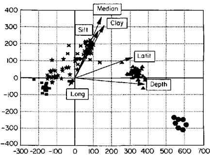
Figure 17. CCA ordination diagram of the five major twin groups based on coeppod composition.
