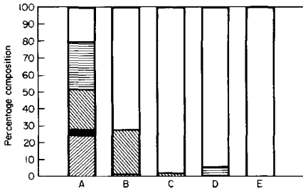
Figure 12. Composition of the North Sea Copepoda per twin group showing importance of exclusively interstitial families in southern twin groups. ▨ Cylindropsyllidae, ■ Cyclopinidae, ▩ Leptastacidae, ▤ Paramesochridae, □ others.
