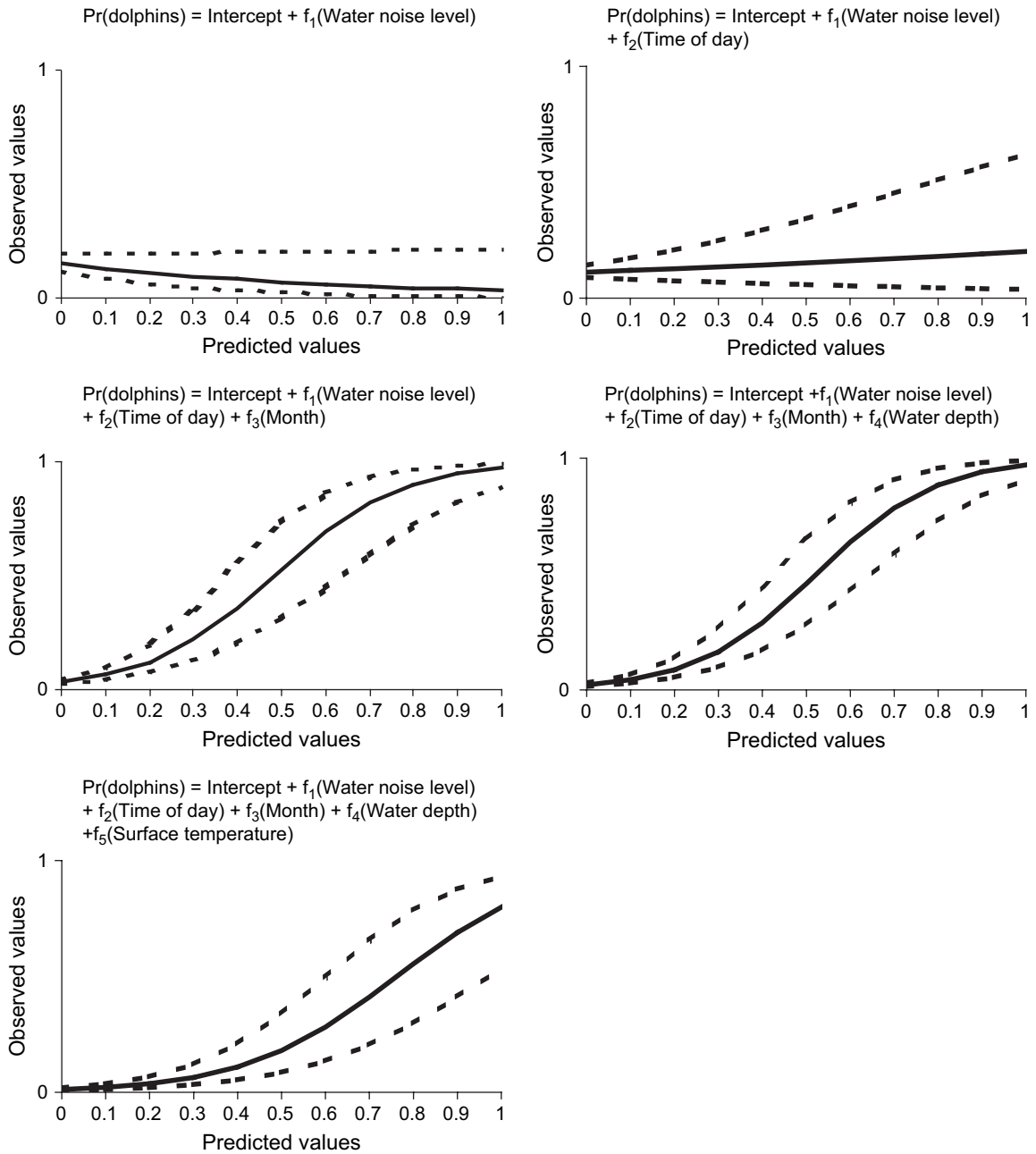
Figure 3. Logistic functions ( \pm s.e.) that represent the relationships between the predicted and observed values of dolphin occurrence, as each term is included to produce a progressively more complex model. The terms included in the model at successive steps are water noise level, time of day, month, water depth, and surface temperature. The “best prediction” model is at the stage when water noise, time of day, month, and water depth are included.
