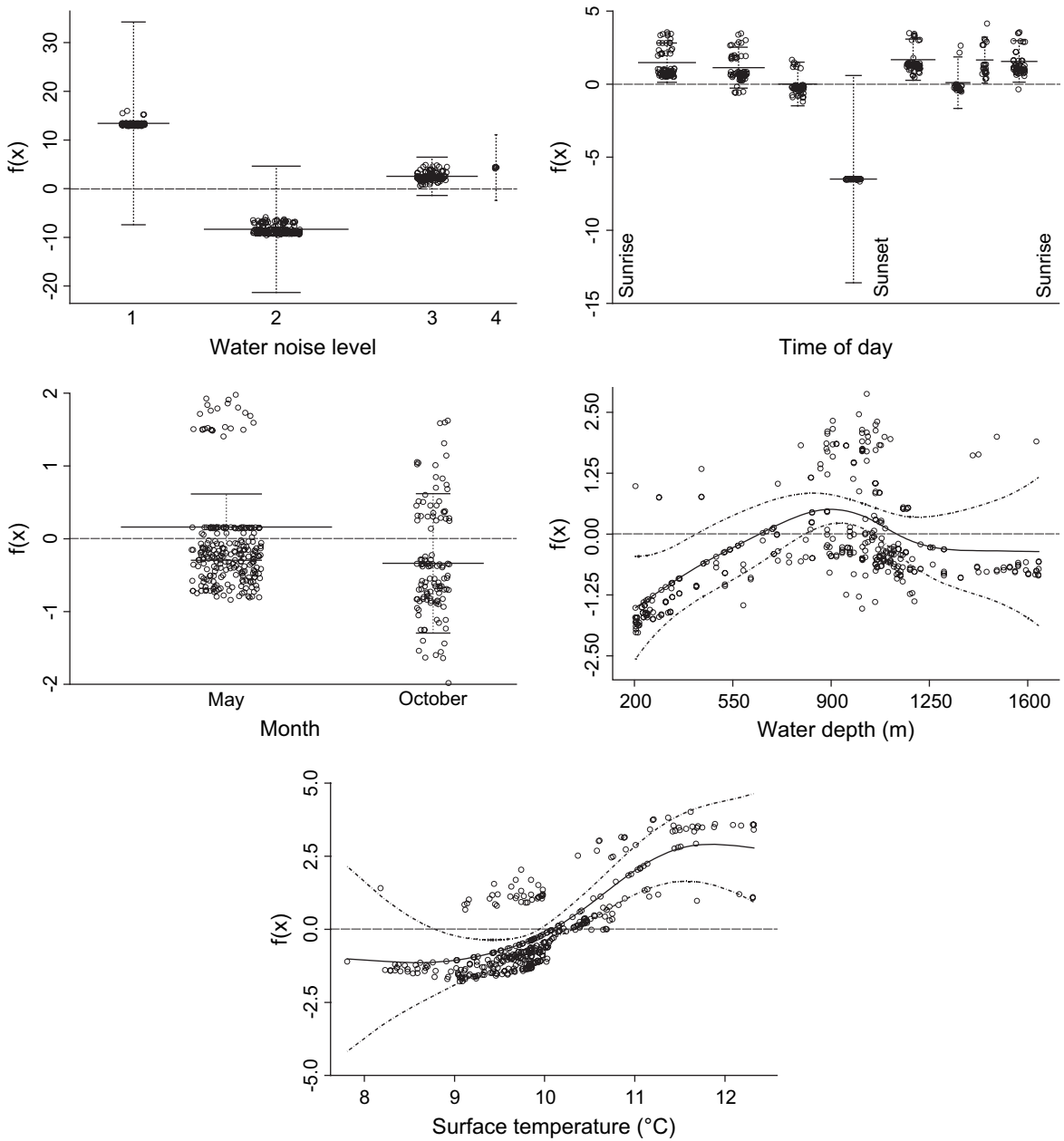
Figure 2. Generalized additive model functions of dolphin encounter rates in relation to environmental variables. The “best prediction” model is at the stage when water noise, time of day, month, and water depth are included. Functions are scaled to the model mean. The dashed lines represent two s.e. bands. The horizontal dashed line represents f(x) = 0 .
