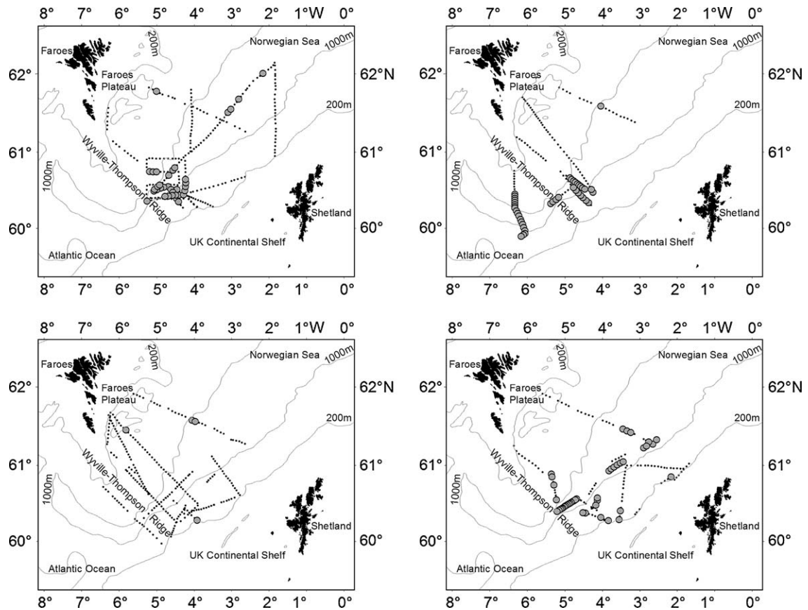
Figure 1. Maps of the study area in the Northeast Atlantic showing the Faroes and Shetland Islands. Surveys lasting 14 days were carried out in May (top left) and October (top right) 2001 and May (bottom left) and October (bottom right) 2002, to build and test environmental models for predicting dolphin distribution in this region. The locations of the acoustic listening stations are shown by the black dots, and the locations where dolphins were heard are shown by the larger grey dots. The dashed contour lines represent water depths of 200 m and 1000 m.
