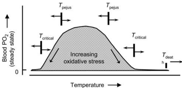
Figure 3. At the cellular level, optimal and suboptimal temperatures are reflected by changes in the rates of aerobic and anaerobic metabolism. Optimal temperatures coincide with the highest levels of PO_2 . Pejus temperatures ( T_{pejus} ) denote the onset of limits in aerobic scope and increased energy demands. Critical temperatures are those where aerobic scope is zero, anaerobic metabolism is measurable and, at the upper T_{critical} , cellular-level stress proteins are produced. At higher temperatures ( T_{death} ), denaturation and death occur. Arrows denote population-specific adaptation (after Pörtner and Knust, 2007).
