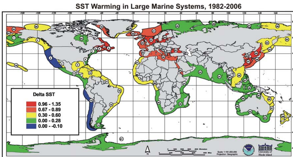
Figure 10. SST trends in the world ocean LMEs, 1982–2006.
