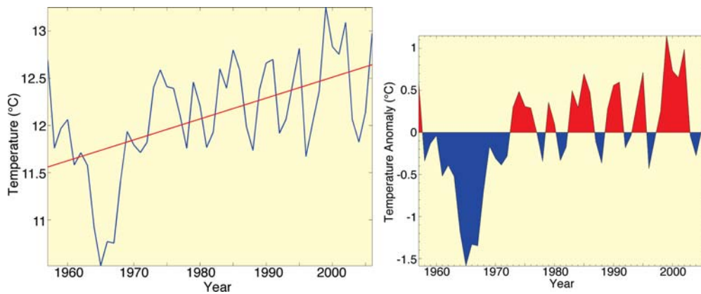
Figure 9. Northeast US continental shelf annual mean SST (left) and SST anomalies (right), 1957–2006, based on the climatology of the UK Meteorological Office’s Hadley Centre.
