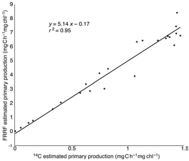
Figure 7. Correlation between the fast-repetition-rate fluorometer (FRRF) and 14 C uptake measured primary productivity for Narragansett Bay samples.
