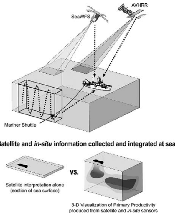
Figure 5. Satellite (SeaWiFS and AVHRR) and in situ information collected by the Mariner Shuttle is integrated at sea.
