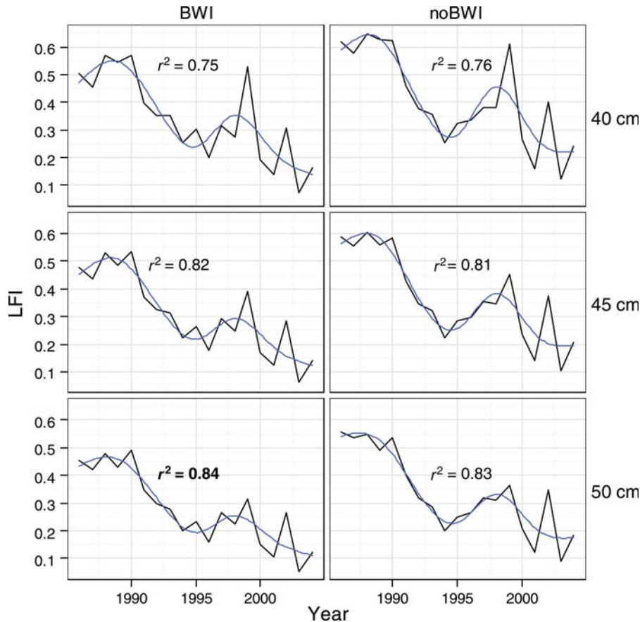
Figure 2. Time-series of the Celtic Sea LFI for two species complexes: North Sea excluding boarfish (noBWI) and North Sea excluding boarfish and including blue whiting (BWI). Three length thresholds for large fish are used (40, 45, and 50 cm). The fitted line is a smoother (sixth order polynomial) with fit ( r^2 ) given for each line. The r^2 for the selected LFI (50 cm, including blue whiting) is shown emboldened.
