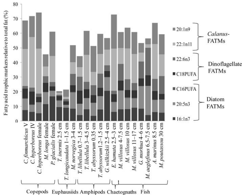
Figure 3. FATMs relative to total fat (%).
