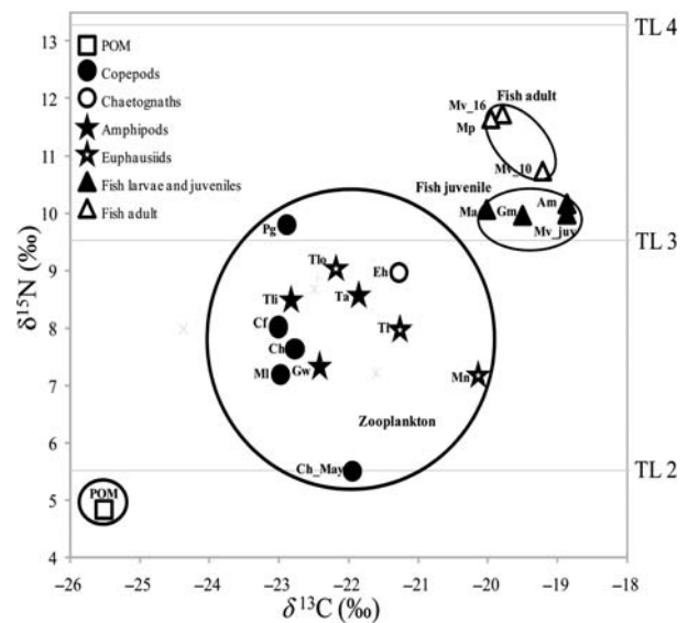
Figure 2. Trophic relationships in the Iceland Sea in August of 2007 and 2008, showing stable isotopes of carbon and nitrogen ( \delta^{13}\text{C} and \delta^{15}\text{N} ) for all species. Values are means, and TL means the trophic level. Abbreviations: Cf, C. finmarchicus ; Ch, C. hyperboreus ; MI, M. longa ; Pg, P. glacialis ; Ti, T. inermis ; Tlo, T. longicaudata ; Mn, M. norvegica ; Tli, T. libellula , TL 1 , 1 cm, TL 4 , 4 cm; Ta, T. abyssorum ; Gw, G. wilkitzkii ; Eh, E. hamata ; Gm, G. morhua ; Ma, M. aeglefinus ; Mv, M. villosus , Mv juv , larvae and juveniles, Mv 10 , 10 cm, Mv 16 , 16 cm, Mv ad , adult (11–16 cm); Mp, M. poutassou ; Am, A. marinus .
