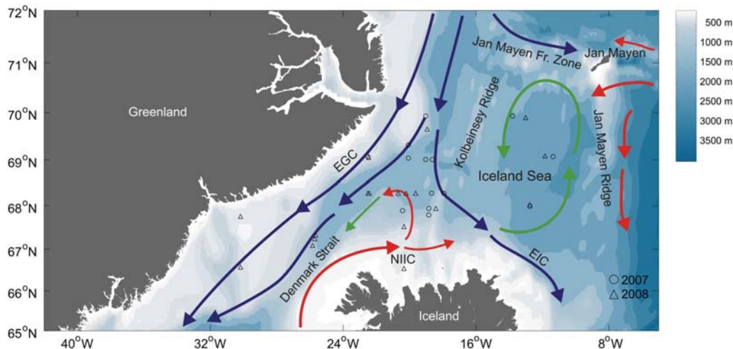
Figure 1. Sampling stations in 2007 (circles) and 2008 (triangles), and circulation in the Iceland Sea, showing Atlantic Water in red, Polar Water in blue, and Arctic Water (a mixture of Polar and Atlantic Water) in green. EGC, East Greenland Current; NIIC, North Icelandic Irminger Current; EIC, East Icelandic Current. Figure courtesy Malin Daase, adapted after Blindheim and Østerhus (2005) and Hunegnaw et al. (2009).
