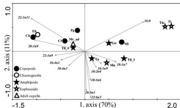
Figure 5. Trophic relationships of adult capelin (11–16 cm) and its potential prey in the Iceland Sea, 2007 and 2008. RDA plot based on moiety (standardized FAs and fatty alcohols) compositions of adult capelin and potential prey. Symbols show the mean values of the respective species. The species were applied as dummy variables (environmental variables) and moieties as response variables. The arrows point in the direction of the steepest increase of the respective moiety. The portion of unconstrained variance accounted for by each axis is shown. Abbreviations: see Figure 2 legend.
