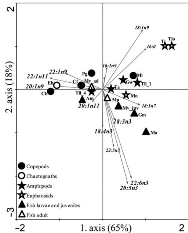
Figure 4. Trophic relationships in the Iceland Sea in August of 2007 and 2008. RDA plot based on moiety values for all species. Symbols indicate the mean values of the respective species. The species were applied as dummy variables (environmental variables) and moieties as response variables. The arrows point in the direction of the steepest increase in the respective moiety. The portion of unconstrained variance accounted for by each axis is shown. Abbreviations: see Figure 2 legend.
