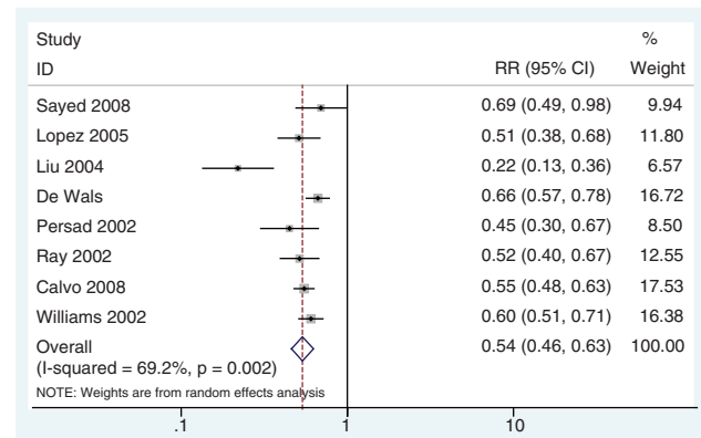
Figure 3 Meta-analysis (random effects) of the effect of folic acid fortification on primary prevention of neural tube defects. Heterogeneity \chi^2 = 22.73 (df = 7), P = 0.002 , I^2 (variation in RR attributable to heterogeneity) = 69.2%; Estimate of between-study variance \tau^2 = 0.0295 , Test of RR = 1: z = 8.01 , P < 0.001
