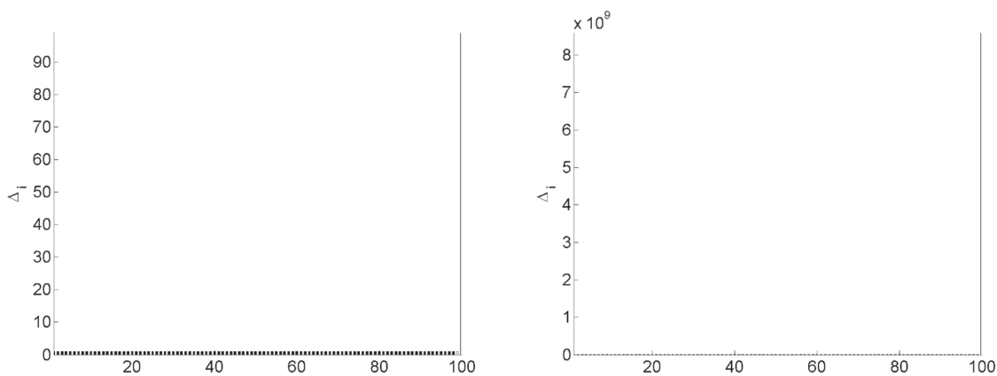
FIG. 9. Constants in (3.6) for problem 4 with history length m = 1 (left plot) and m = 5 (right plot).
