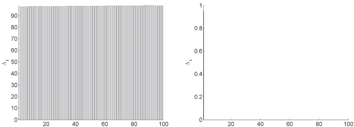
FIG. 10. Constants in (3.6) for problem 5 with history length m = 1 (left plot) and m = 5 (right plot).
