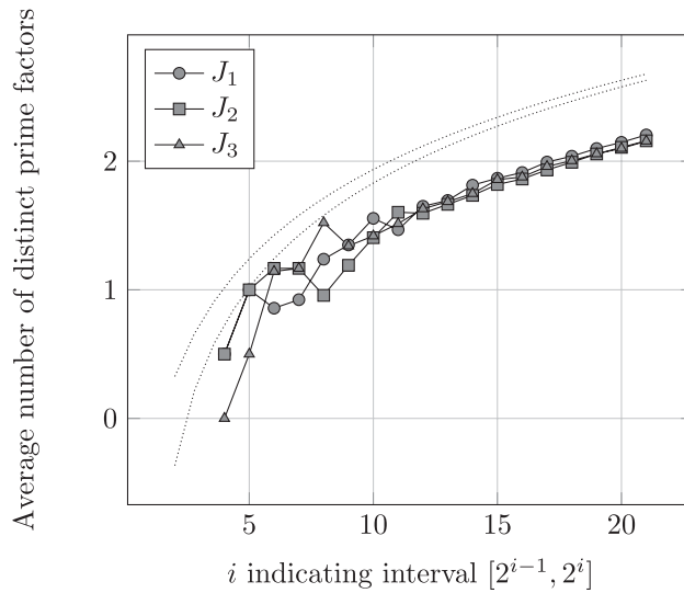
Fig. 3. Average number of v(a_{1,p}) for J_1 , J_2 , and J_3 , in the intervals [2^{i-1}, 2^i] , i = 2, \dots, 21 . For comparison, the graphs of \log(\log(2^i)) and \log(\log(2^{i-1})) are shown in dotted lines.
