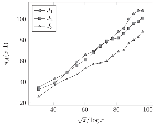
Fig. 2. Values of \pi_A(x, 1) versus \sqrt{x}/\log x for various Jacobians of hyperelliptic curves.
