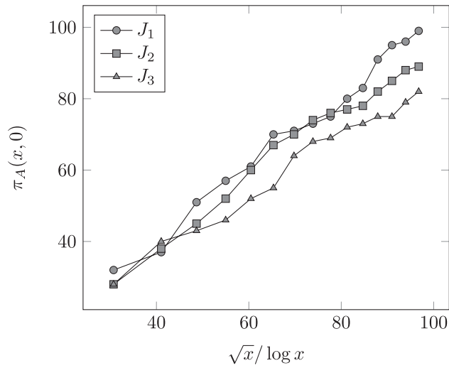
Fig. 1. Values of \pi_A(x, 0) versus \sqrt{x}/\log x for various Jacobians of hyperelliptic curves.
