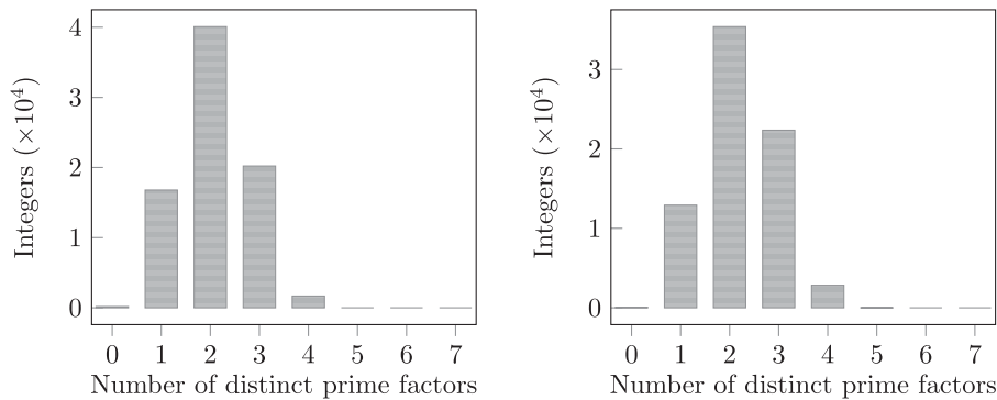
Fig. 4. Histograms of \nu(a_{1,p}) for J_1 ; on the left, the data are for primes p < 2^{20} , and on the right, the data are for primes 2^{20} < p < 2^{21} . Primes of bad reduction and primes for which the trace is zero are excluded.
