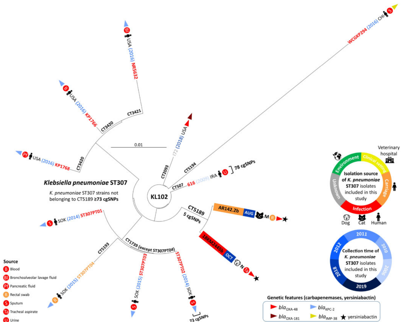
Figure 3. Phylogenetic neighbour-joining tree based on the wgMLST of CPKp ST307 causing nosocomial infections ( n=1 ), carriage CPKp ( n=1 ) and other K. pneumoniae from the NCBI database ( n=10 ) with their respective features. The CPKp described in this study are highlighted in arcs and they are coloured depending on their source and year of isolation. Carbapenemase genes are displayed as triangles and the colour relates to specific genes (as displayed by the legend). Details regarding the source are shown according to the legend. Regarding the capsular type, all strains included herein exhibited KL102. CTs are also displayed for every strain included. The other K. pneumoniae isolates were obtained from the NCBI database ( n=10 ) using the search tool assembly. Only submissions with fully assembled chromosomes were included in the study (accessed on 5 January 2020). The tree was generated and drawn using SeqSphere+ v601 for the comparison of 5124 genes among all the genome sequences included ( n=12 ) based on 'pairwise ignoring missing values; % column differences'. CHI, China; IRA, Iran; SOK, South Korea. This figure appears in colour in the online version of JAC and in black and white in the printed version of JAC.
