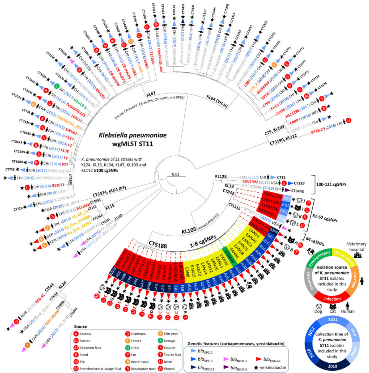
Figure 2. Phylogenetic neighbour-joining tree based on the wgMLST of CPKp ST11 causing nosocomial infections ( n=14 ), environmental CPKp ( n=15 ), CSKp ( n=4 ) and other K. pneumoniae from the NCBI database ( n=67 ) with their respective features. The CPKp described in this study are highlighted in arcs and they are coloured depending on their source and year of isolation, as shown by the legend. Carbapenemase genes are displayed as triangles and the colour relates to specific genes (as displayed by the legend). Details regarding the source are shown according to the legend. Regarding the capsular type, a minimum score of ‘good’ (PF, perfect; VH, very high; H, high) from KAPTIVE was applied as a threshold; when the result was lower, the capsular type was not included in the figure. CTs are displayed for every strain included in the analysis. The cgSNPs were included for the CPKp strains included in this study (1–8 cgSNPs), the closest relative human strain (KP38731) and the strains belonging to the closest clade (JM45, CAV1392 and SCKP020046). The other K. pneumoniae strains were obtained from NCBI ( n=67 ) using the search tool assembly. Only submissions with fully assembled chromosomes were included in the study (accessed on 5 January 2020). The tree was generated and drawn using SeqSphere+ (v601) for the comparison of 4894 genes among all the genome sequences included ( n=100 ) based on ‘pairwise ignoring missing values; % column differences’. NOR, Norway; CHI, China; GER, Germany; GRE, Greece; CAN, Canada; TAI, Taiwan; JAP, Japan. This figure appears in colour in the online version of JAC and in black and white in the printed version of JAC.
