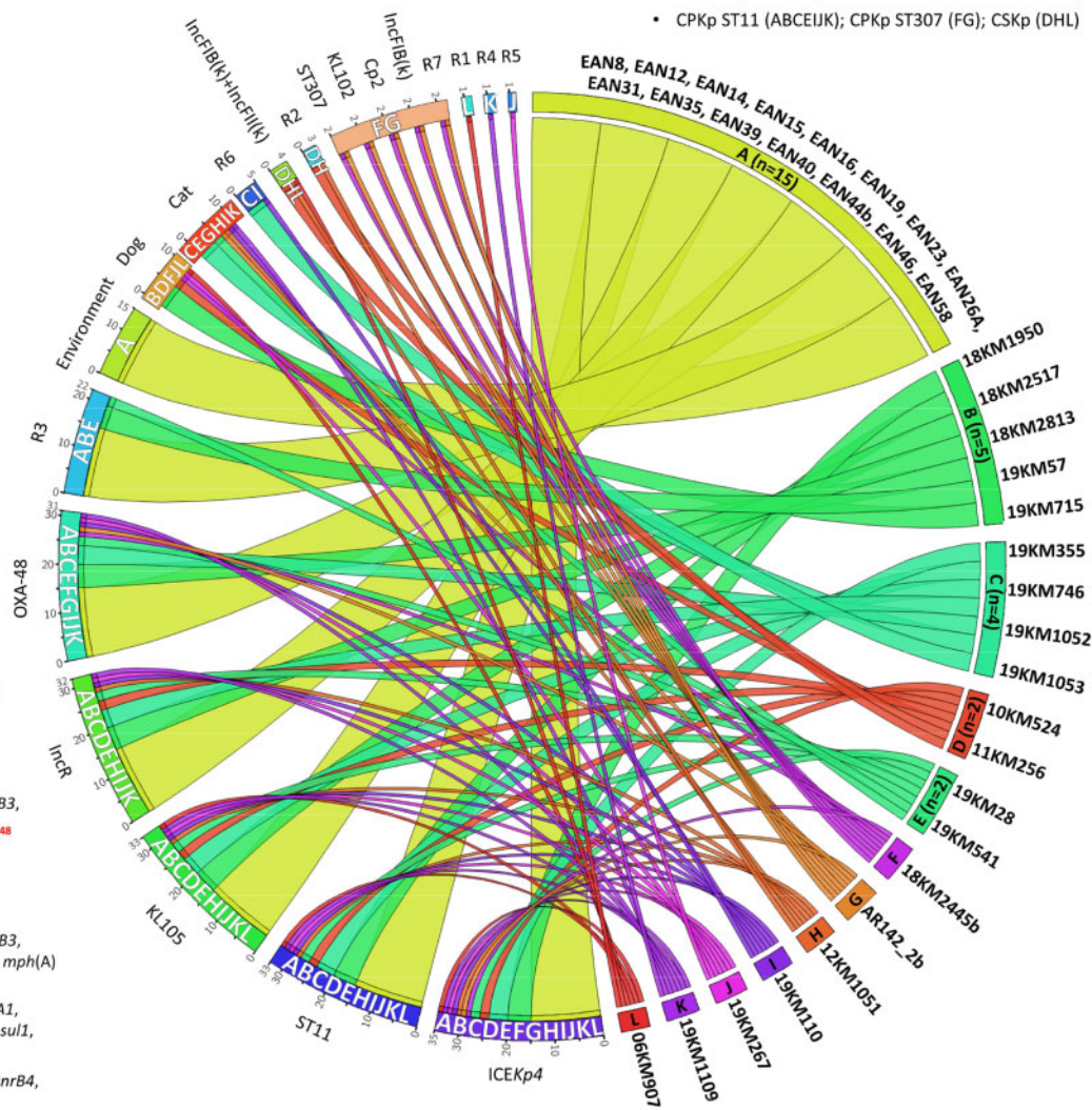
Figure 1. Features of CPKp (n = 31) and CSKp (n = 4) included in this study. Circos diagram showing the 35 strains (right) and the connection to their respective features (left). The strains were clustered into 12 groups (A, B, C, D, E, F, G, H, I, J, K and L) based on their similarity (rounded rectangles and black bold font, right side). When a strain group presents a specific feature, the letter representing the group is displayed within the rounded rectangle of the respective feature (white bold font, left side). The resistance genotypes of the strains were divided into seven classes, as displayed in the legend; red and bold formatting highlight the most relevant genes. The outer edge of the rounded rectangle of each feature shows how many strains possess that feature. This figure appears in colour in the online version of JAC and in black and white in the printed version of JAC.
