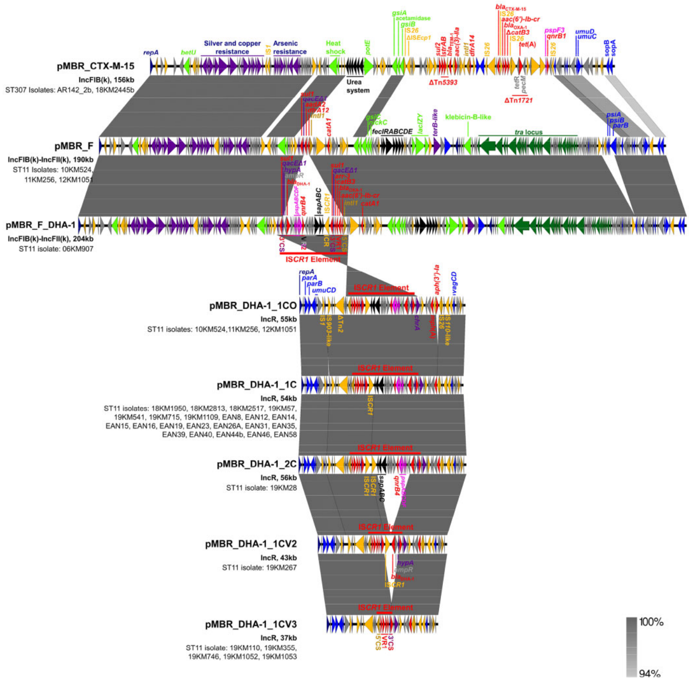
Figure 4. Linear comparison map of the MDR plasmids found in CPKp and CSKp strains from this study. The figure was obtained from Easyfig and the minimal size for BLASTn comparisons was set at 2000 bp to facilitate the visualization of the structural similarities and differences. The classical ISCR1 element is composed of the 5' conserved region (5'CS), variable region 1 (VR1), common region, variable region 2 (VR2) and the 3' conserved region (3'CS). Genes are indicated with arrows and are coloured depending on their gene functional classification as follows: ARGs are red; transposases are orange; integrases are dark orange; genes related to conjugation are dark green; genes related to increased fitness are light green; disinfectant and heavy metal resistance genes are purple; phage-related genes are pink; partition, modification and stability systems are in blue; replication genes are dark blue; putative genes that can increase virulence are black; and other genes are grey. This figure appears in colour in the online version of JAC and in black and white in the printed version of JAC .
