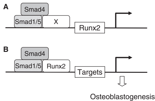
Fig. 1 Activated Smad1/5 and Smad4 regulate Runx2 expression (A), and subsequently, associate with Runx2 to regulate target genes necessary for osteoblastogenesis (B). An unidentified transcription factor (X) is implicated in BMP-mediated induction of Runx2.
