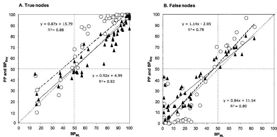
FIG. 2.—Linear correlation between maximum likelihood bootstrap percentages ( BP_{ML} ) and Bayesian posterior probabilities (PP; circles) or bootstrapped Bayesian posterior probabilities ( BP_{Bay} ; triangles) in 25 simulated data sets. “True nodes” are nodes that were present in the model topology used to simulate the data sets and “false nodes” are nodes that were not in the model topology. The dotted line represents a slope of 1—with equality of BP_{ML} and PP or BP_{Bay} —while dashed and plain lines represent PP = f(BP_{ML}) and BP_{Bay} = f(BP_{ML}) regression lines, respectively. All axes represent node support as percentages. The phylogram used for the simulation was (A:0.043143,(B:0.027559,(C:0.018247,D:0.024211):0.003601):0.011055,(E:0.005704,(F:0.010024,G:0.006528):0.000708):0.021913):0.003809) with branch lengths issued from the xenarthran data set, and taxa A–G corresponding to Dasytus kappleri , Tolypeutes matacus , Cabassous unicinctus , Priodontes maximus , Euphractus sexcinctus , Chaetophractus villosus , and Zaedyus pichiy , respectively.
