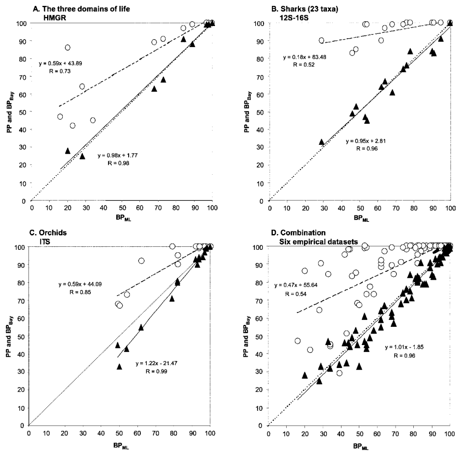
FIG. 1.—Linear correlation between maximum likelihood bootstrap percentages ( BP_{ML} ) and Bayesian posterior probabilities (PP; circles) or bootstrapped Bayesian posterior probabilities ( BP_{Bay} ; triangles) for empirical data sets. The dotted line represents a slope of 1—with equality of BP_{ML} and PP or BP_{Bay} —while dashed and plain lines represent PP = f(BP_{ML}) and BP_{Bay} = f(BP_{ML}) regression lines, respectively. All axes represent node support as percentages. See table 1 for further information regarding data sets.
