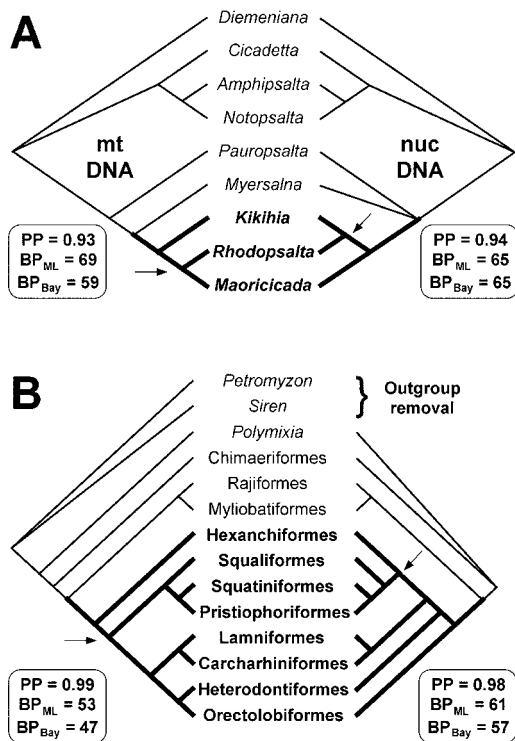
FIG. 3.—Illustration of the effect of the bootstrapped Bayesian approach in two cases of apparently conflicting nodes based on Bayesian posterior probabilities. (A) Conflict between maximum likelihood phylograms for mitochondrial (mtDNA) and nuclear (nucDNA) genes of Pacific Cicada genera (original data from Buckley et al. 2002). (B) Conflict about the position of Hexanchiformes within Elasmobranchs between maximum likelihood phylograms of the chondrichthyan 12S and 16S rRNA data sets differing only by the number of outgroup taxa (i.e., rooting with and without Petromyzon and Siren [original data from Douady et al. in press]). PP: Bayesian posterior probability; BP ML : maximum likelihood bootstrap percentage; BP Bay : Bayesian bootstrapped posterior probability. The arrows indicate apparently conflicting nodes for which PP, BP ML , and BP Bay are given. Thick branches connect taxa (bold names) involved in the apparent topological conflicts.
