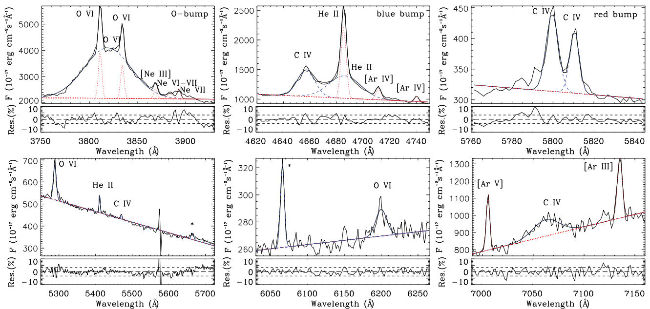
Figure 4. Multicomponent Gaussian fits to the O-bump (top left), blue bump (top centre), and red bump (top right) panels. The bottom panels show other WR features in the spectrum of WD 0722+295. The (blue) dashed lines represent the fits to the broad (stellar) features, the (red) dotted line the fits to the nebular emission, and the (black) line the sum. Residuals are shown at the bottom of each panel.
