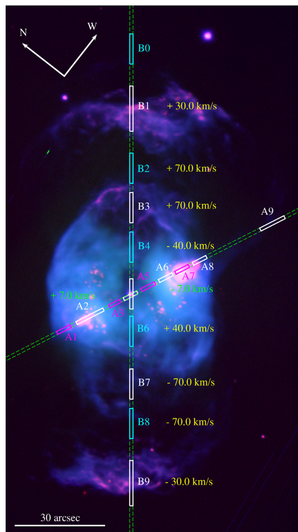
Figure 2. CFHT colour-composite ([O III] – blue, H \alpha – green, [N II] – red) image of NGC 2371. The (green) dashed line regions represent the slit positions obtained from our INT IDS observations. The PA for the slits are 65° (Slit A – minor axis) and 128° (Slit B – major axis). Different extraction regions are labelled and shown with different colours. The green and yellow velocity measurements correspond to the A2, A7, and B1–B9 extraction regions. See text for details.
