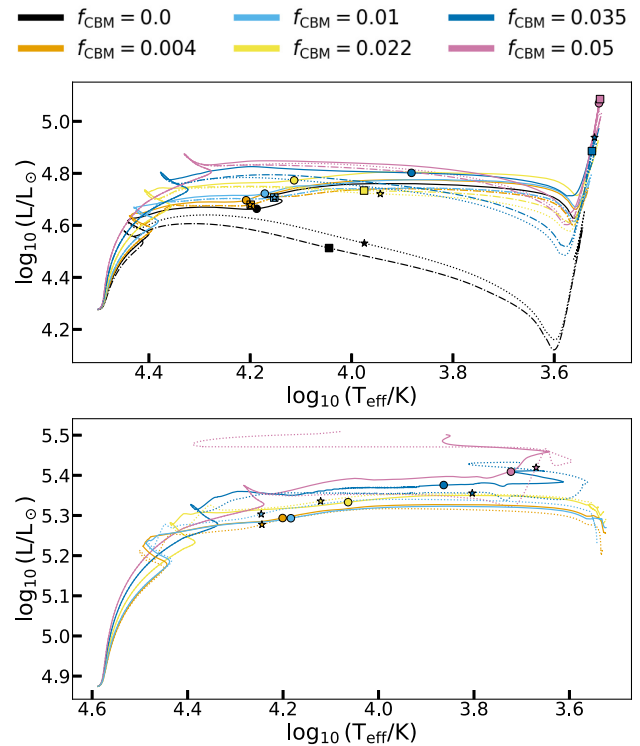
Figure 11. The HRD for various calculations of models with initial masses of 15 (top) and 25M_{\odot} (bottom), all with f_0 = 0.002 . The solid lines indicate Schwarzschild models and all the others are Ledoux models with either \alpha_{\text{sc}} = 0.4 (dotted line) or \alpha_{\text{sc}} = 0.004 (dash-dotted line). The colour scheme indicates the amount of CBM. The markers show the location where helium burning is ignited in the core (0.3 per cent of the helium left after core hydrogen depletion is burnt). The different marker styles indicate the different boundary criteria used in the calculation, where circles indicate the Schwarzschild criterion and the others are Ledoux models with \alpha_{\text{sc}} = 0.004 (square) or \alpha_{\text{sc}} = 0.4 (star).
