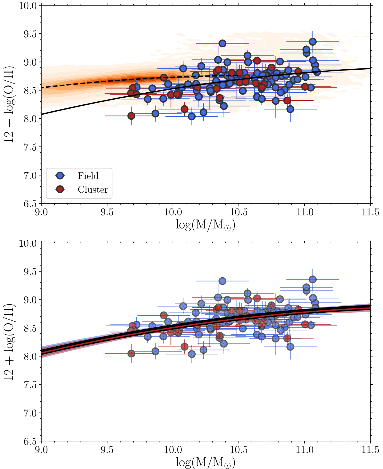
Figure 7. Top: Mass–metallicity (MZ) relation for K-CLASH star-forming galaxies. We use the polynomial conversion of Pettini & Pagel (2004) to infer 12 + \log(O/H) from measurements of [N II]/H\alpha . Cluster galaxies are shown in red with field galaxies in blue. The orange contours show local star-forming galaxies from the 12th data release of the Sloan Digital Sky Survey, with emission line measurements from Thomas et al. (2013) and stellar masses from Maraston et al. (2009). The solid and dashed lines show a polynomial fit to the K-CLASH and SDSS galaxies of the form of equation (2), following Maiolino et al. (2008). Bottom: The K-CLASH sample split by environment. The red and blue lines show best-fitting polynomials from equation (2) to the cluster and field galaxies, respectively. These fits are derived from a hierarchical Bayesian model: see equation (3) for details. The shaded regions represent the one \sigma uncertainties around the fits. We note that we have already removed galaxies with a large [N II]/H\alpha ratio [and therefore large 12 + \log(O/H) values] in their central spectrum, since they are likely to contain an AGN (see Section 2.1).
