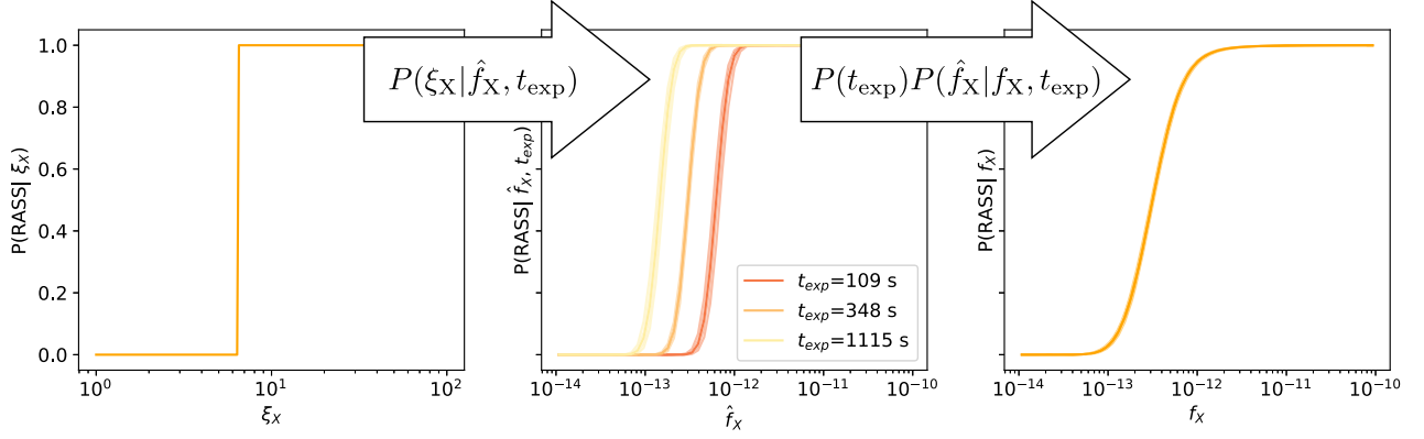
Figure 1. Schematic representation of the construction of the X-ray selection function: in the space of detection significance \xi_X (left), the selection function is simply a step function. Objects above the selection cut are selected, and objects below not. Using the stochastic mapping P(\xi_X|\hat{f}_X, t_{\text{exp}}) between detection significance and measured flux \hat{f}_X at a given exposure time t_{\text{exp}} , we construct the selection function in the space of measured flux \hat{f}_X and exposure time t_{\text{exp}} (centre). Accounting for the solid angle weighted exposure time distribution P(t_{\text{exp}}) and the measurement uncertainty on the flux P(\hat{f}_X|f_X, t_{\text{exp}}) , results in the X-ray selection function in the space of intrinsic flux f_X (right). The latter is usual determined in image simulations making specific assumption on the cluster morphology. In contrast, our method empirically determines the mapping between detection significance and measured flux, thereby accounting for the real morphological variation in the cluster population as well as its uncertainty.
