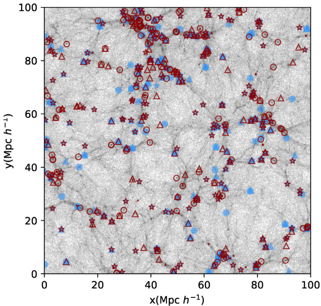
Figure 12. Distribution of galaxies with a number density of 10^{-2}h^3 \text{Mpc}^{-3} , on top of the smooth underlying dark matter distribution (grey). This slice of 10h^{-1} \text{Mpc} thickness is taken from the MS-W7 simulation at z = 0.99 . The red symbols show fixed number density galaxies selected with a single cut in stellar mass (the circles), SFR (the triangles), or L[O II] (stars), while the blue ones show those fixed number density DEEP2 galaxies selected with an extra cut on the mentioned properties. The area of the symbols is proportional to the \log_{10}(L_{[\text{OII}]}) .
