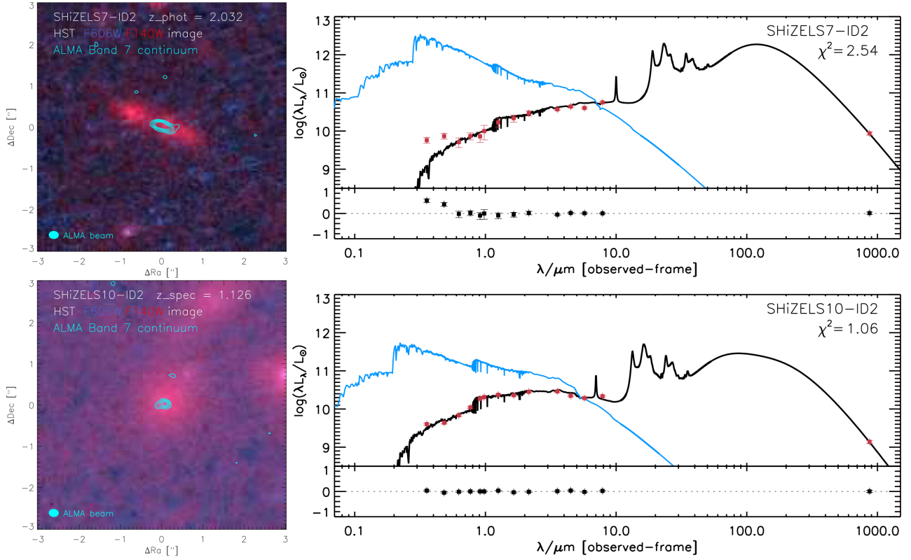
Figure D1. Left-hand panels: Fake colour image (blue for F606W and red for F140W) with ALMA contour ( 3, 4, 5, 6, 7 \times rms). Right-hand panels: Redshifts and SEDs taken from Mehta et al. (2018) as well as our new ALMA observations are shown in red dots. We fit the SED using MAGPHYS (da Cunha et al. 2008). The initial stellar spectra are shown in blue lines, and the model SED after considering the dust extinction are shown in black lines.
