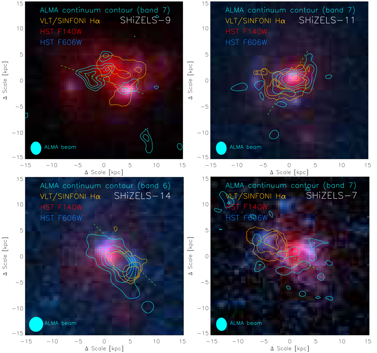
Figure 1. The HST F606W (blue) and F140W (red) true-colour composite images, including ALMA continuum contours (cyan) and H \alpha contours (orange). Contour levels are shown at 2\sigma , 3\sigma , 4\sigma , and 5\sigma . The ALMA synthesized beam is shown in the lower left corner. The green dash lines show the direction of major kinematic axis ( PA_{\text{vel}} , see the velocity map in Gillman et al. 2019). The three different tracers of star formation are clearly highlighting very different regions.
