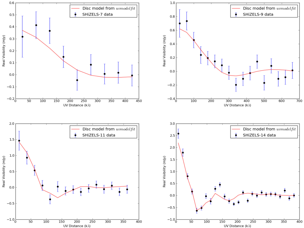
Figure 5. The uv -real visibility diagrams of the ALMA detected targets. The black dots and blue error bar are obtained from the ALMA data while the red lines are the fitting results by disc model in the CASA task UVMODELFIT .
