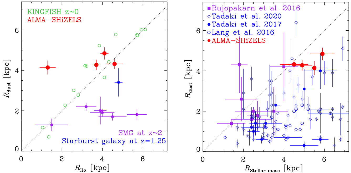
Figure 7. Left-hand panel: Comparison of the half-light radii measured in the ALMA continuum imaging with respect to those measured in H\alpha (Swinbank et al. 2012b; Molina et al. 2017). We also overplot the Herschel 350- \mu\text{m} and narrow-band H\alpha radii (obtained after convolving both to the same resolution) from the KINGFISH (Kennicutt et al. 2011) and Spitzer Infrared Nearby Galaxies Survey (SINGS) projects (Kennicutt et al. 2003; Dale et al. 2005, 2007). Our high-redshift galaxy sample shows a broadly similar behaviour as is seen in these local galaxies, except SHiZELS-11, which shows a significantly larger radius in the FIR than in H\alpha . We also show the recent ALMA-resolved SMG sample at z \sim 2 (Chen et al. 2020) and one starburst galaxy (GOODSN-18574) at z = 1.25 (Nelson et al. 2019). Right-hand panel: The stellar mass size as derived from the HST F140W image compared to the FIR size as derived from the ALMA observations. We show the H\alpha selected main-sequence star-forming galaxies at redshift about 2.2–2.5 by Tadaki et al. (2017), the star-forming galaxies presented by Rujopakarn et al. (2016), the z \sim 2 SMGs from Lang et al. (2019), and the massive star-forming galaxy sample at z \sim 2 from Tadaki et al. (2020). The dot line shows the one-to-one relation. Our targets are roughly the largest galaxies in both rest-frame optical band and FIR radius and may evolve into massive disc galaxies.
