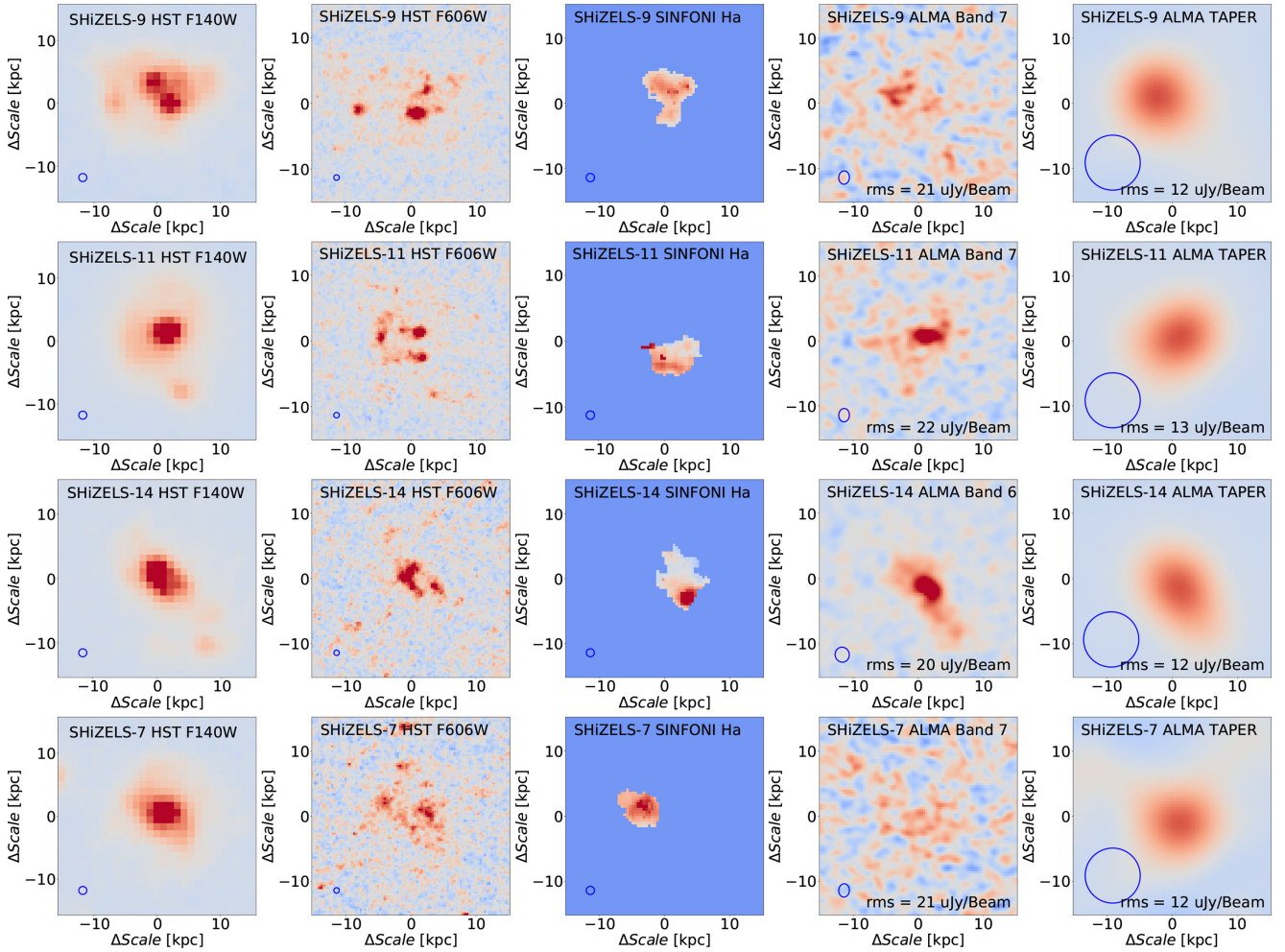
Figure A1. Postage stamp (30 kpc \times 30 kpc) images for the SHiZELS galaxies presented in this work. From left to right images: HST F140W, HST F606W, VLT/SINFONI H\alpha moment-0, Briggs weighting (ROBUST = 0.5) ALMA continuum at \sim 355\text{-}\mu\text{m} rest frame, and tapered ALMA image (synthesized beam of \sim 1'' ) to highlight extended emission. The image shows the complexity of the different phases of the ISM in these high-redshift galaxies.
