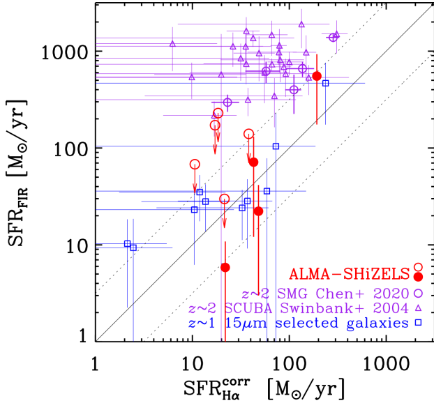
Figure 3. The total SFRs derived from the extinction-corrected H \alpha (equation 3) and FIR luminosities for z \sim 2.23 and z \sim 1.47 samples, respectively. We show the ALMA-detected targets as filled red circles and the ALMA non-detected targets as open red circles. We compare our findings with previously observed SMGs at z \sim 2 from Swinbank et al. (2004) and Chen et al. (2020). A sample of 15- \mu\text{m} selected galaxies (at z \sim 1 ) presented by Franceschini et al. (2003) are also shown. The dotted lines show 0.5 dex above and below the solid line.
