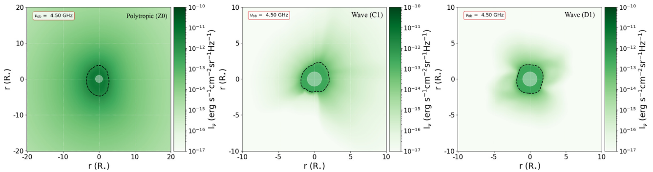
Figure 8. Radio intensities of the polytropic wind, Alfvén-wave-driven wind with a ZDI map, and Alfvén-wave-driven wind with a dipole, respectively, shown in Figs 3–5. Plots from the Alfvén-wave-driven wind models are zoomed in to [-10, 10] R_* to display more detail. It is evident from these plots that the density decay in the Alfvén-wave-driven winds has a significant effect on the radio flux density emitted from the wind. The black dashed contour shows the optically thick surface of \tau = 0.399 at 4.5 GHz, which delineates the region within which half of the emission originates (Panagia & Felli 1975).
