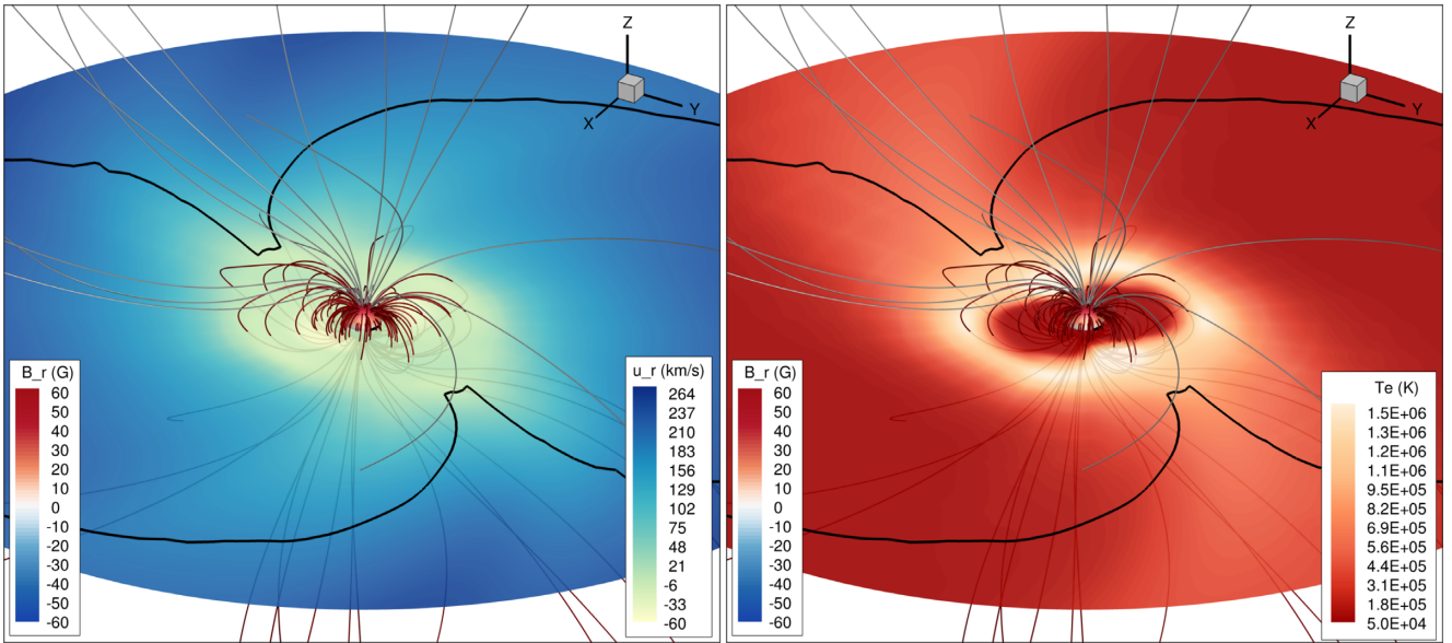
Figure 5. Model D1, one of the Alfvén-wave-driven wind simulations, with a dipolar field of B_{\text{dip, max}} = 60 G, as in Fig. 3. The circular plane shown above extends from -30 to 30 R_* across its diameter.
