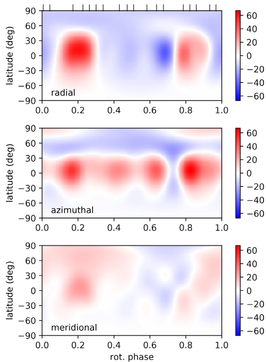
Figure 2. Large-scale magnetic field geometry of \lambda And, as reconstructed with the ZDI method. From top to bottom, the three panels show the radial, azimuthal, and meridional components of the photospheric magnetic field (in Gauss). The observed rotational phases are shown as vertical ticks above the radial field map.
