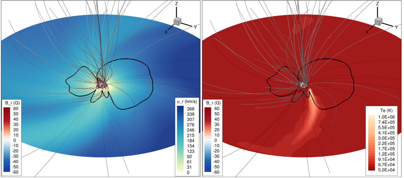
Figure 4. Model C1, one of the Alfvén-wave-driven wind simulations, with the ZDI map set as the inner boundary for the magnetic field, as in Fig. 3. The circular plane shown above extends from -30 to 30 R_* across its diameter.
