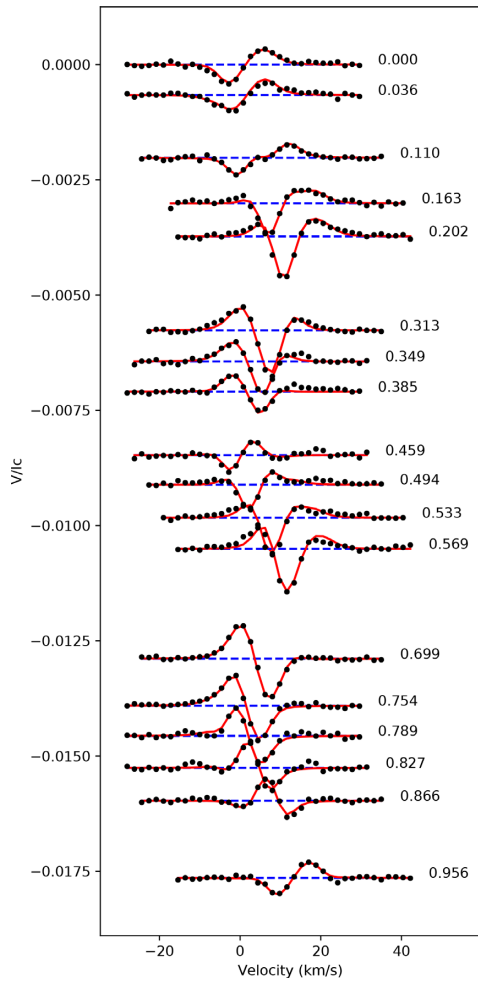
Figure A2. The same as Fig. A1, but for Stokes V profiles.
