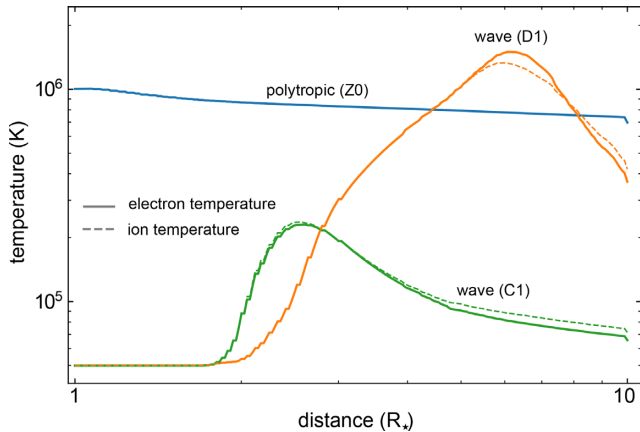
Figure 6. The averaged temperature around the equator of three simulations shown in blue (polytropic, Fig. 3), green (wave-driven C1 , Fig. 4), and orange (wave-driven D1 , Fig. 5), respectively. Solid lines are the electron temperature, while the ion temperature is shown by the dashed lines.
