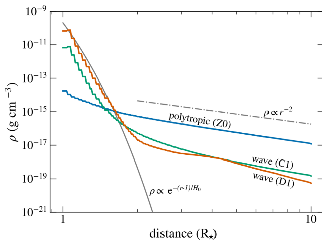
Figure 9. In this plot we show the averaged density around the equator of three simulations shown in blue (polytropic, Fig. 3), green (wave-driven C1, Fig. 4), and orange (wave-driven D1, Fig. 5), respectively. The Alfvén-wave-driven winds display hydrostatic behaviour close to the stellar surface and we see an exponential decay with a scale height of H_0 = 0.05 R_* . Grey lines show examples of r^{-2} (dot-dash) and exponential decay (solid).
