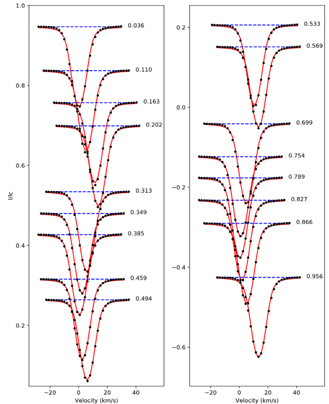
Figure A1. Stokes I LSD pseudo-profiles of \lambda And (black points), overplotted with the set of synthetic Stokes I profiles produced by the ZDI model (red line). The profiles are vertically shifted for display clarity. The dashed blue lines show the continuum level, and the phases of observation are indicated on the right of every profile, assuming a 54 d rotation period, and taking our first observation as phase origin.
