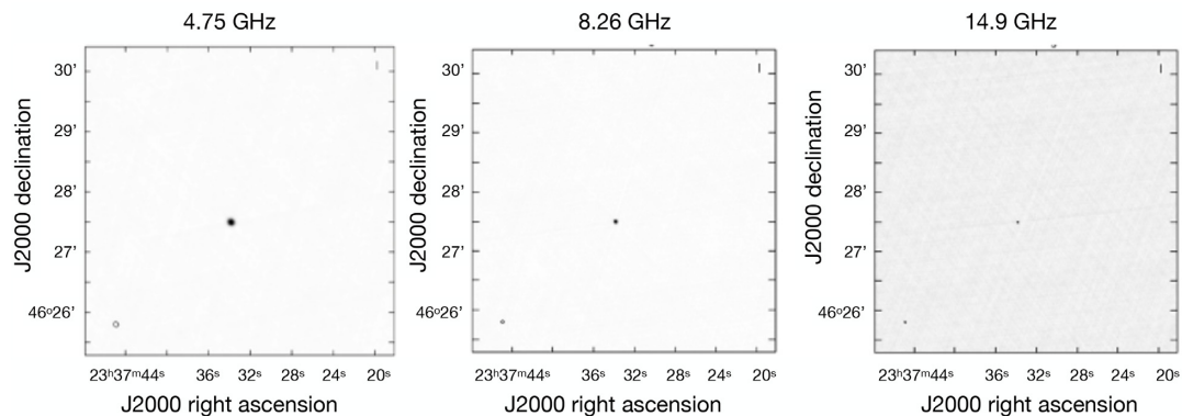
Figure 7. VLA observations of \lambda And from 1998 December 12 (program AN0083) at the C, X, and U bands (4.75, 8.26, 14.9 GHz) during an active state of the star.
