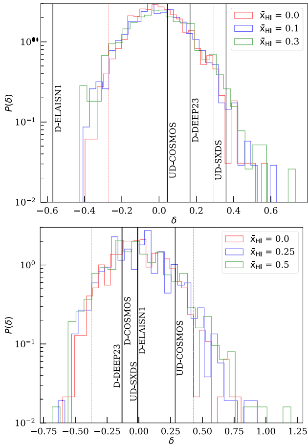
Figure 4. Cosmic variance in the surface density of SILVERRUSH-sized fields of view. Here, we show the probability distribution of the surface density contrast, \delta = \Sigma / \langle \Sigma \rangle - 1 . The top and bottom panels correspond to z = 5.7 and z = 6.6 , respectively. The red, blue, and green histograms represent our models with different global neutral fractions. The vertical black lines represent \delta measured from the publicly available SILVERRUSH catalogues (Shibuya et al. 2018), with uniform luminosity and colour cuts applied. The red, thin-dashed lines show the 2\sigma range of our surface density distribution in a completely ionized scenario. Black lines are annotated with individual field names. A more neutral IGM yields only a slight increase in the cosmic variance. Our model distributions are consistent with the data, aside from D-ELAISN1, which is likely affected by poor seeing (Konno et al. 2018).
