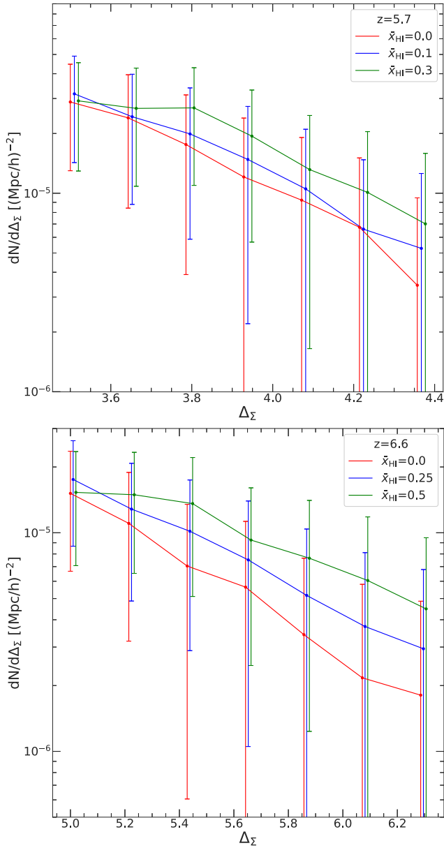
Figure 9. The POF, dN/d\Delta_\Sigma , or number of peaks per unit area, per unit surface overdensity, \Delta_\Sigma = \Sigma/(\Sigma) . For this statistic, peaks are identified as connected sets of pixels satisfying a minimum overdensity threshold, as well as a minimum LAE occupancy (see main text for details). Error bars show the 1\sigma dispersion from cosmic variance in an expanded (10-field) SILVERRUSH-like survey. At fixed \langle\Sigma\rangle , the overdense LAE peaks are more numerous in models with higher neutral fraction.
