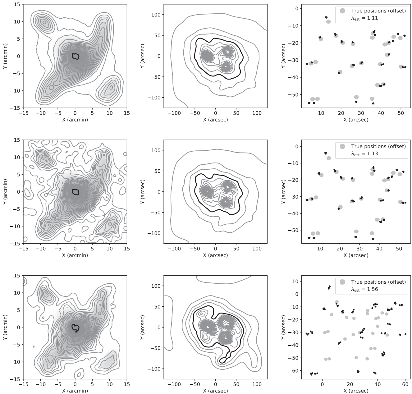
Figure 13. The three rows correspond to inputs (A), (B), and (C), obtained when the mass sheet basis function is not used. The left-hand panels show the wide area reconstruction, mainly due to the weak lensing data, where the background shows the shape of the true mass density for comparison. To make the small features better visible, a logarithmic grey-scale was used. The centre panels show the reconstructions of the strong lensing regions, all having quite similar features. While the overall shapes are similar, the contour spacing in scenario (C) shows a steeper mass map. The right-hand panels show the back-projected images in each case. While consistent source positions as well as the source plane scales could be recovered for scenarios (A) and (B), the scales differing by 11 and 13 per cent, respectively, for scenario (C) neither do the back-projected images overlap well, nor is the scale of the back-projected images consistent with the true source plane scale. The size of the filled grey circles is again 2 arcsec.
