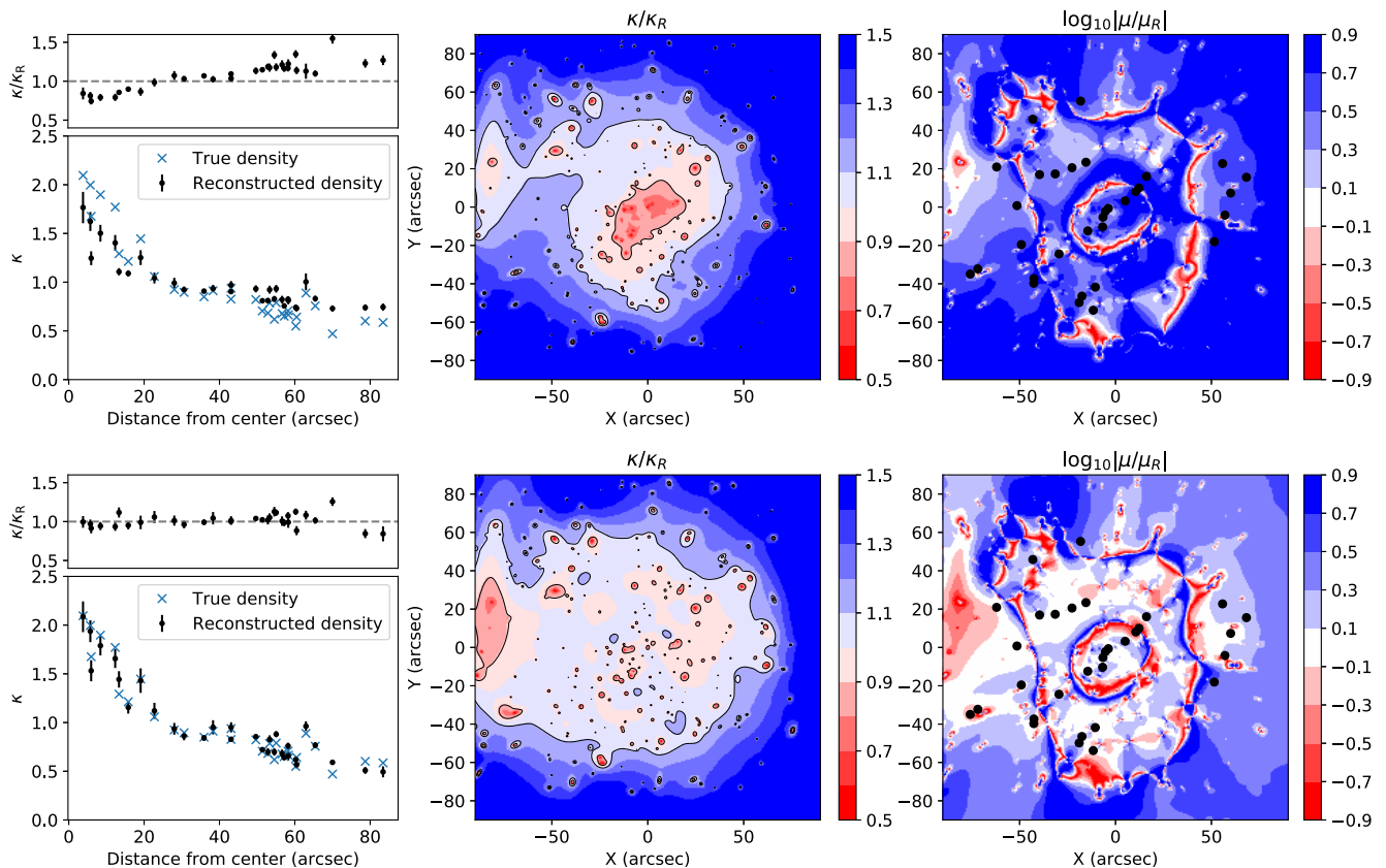
Figure 3. In each of the three panels, the top figure corresponds to the solution obtained with \text{fitness}_{\text{TD},2009} and the bottom figure to the one obtained with \text{fitness}_{\text{TD},\text{NoSrc}} . Left-hand panel: the larger plots show both input and recovered densities measured at the positions of the images, while the smaller ones show the fraction of the recovered density \kappa to the real density \kappa_R . For visualization purposes, only the distance of a point to the coordinate centre is shown on the horizontal axis. Whereas the newly proposed fitness measure yields densities that match the true ones well, the other one produces solutions that are less steep, and that have a more prominent density offset, i.e. that differ by the MSD. Centre panel: these maps show the \kappa/\kappa_R fraction in the region under consideration. The solid black line marks the 10 per cent boundaries. While the \text{fitness}_{\text{TD},2009} solution has clear difference in both the central and outer regions, similar as what can be seen in the left-hand panel, the solution obtained with the new fitness measure is well constrained over a large area. Right-hand panel: these plots compare the magnification of the recovered lens model \mu to the true magnification \mu_R , both for a redshift of z = 9 . The consistently larger magnification for the older fitness measure is again a sign of the MSD. The new \text{fitness}_{\text{TD},\text{NoSrc}} on the other hand produces a much more consistent map.
