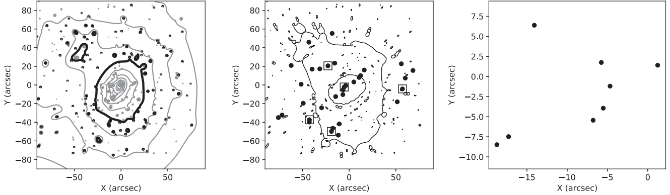
Figure 1. For the time delay test, an existing model for Abell 1689 was used (Limousin et al. 2007), the mass distribution of which is depicted by contours in the left-hand panel. The solid lines indicate \kappa = 1 (for a source redshift of z = 3 ); the spacing between contours is \Delta\kappa = 0.2 . The filled circles in the centre panel show the 32 image positions generated by the eight point sources in the right-hand panel; the squares indicate the multiple-image system that is used in the left-hand panel of Fig 4. The critical lines shown in the centre panel also refer to a redshift of z = 3 .
