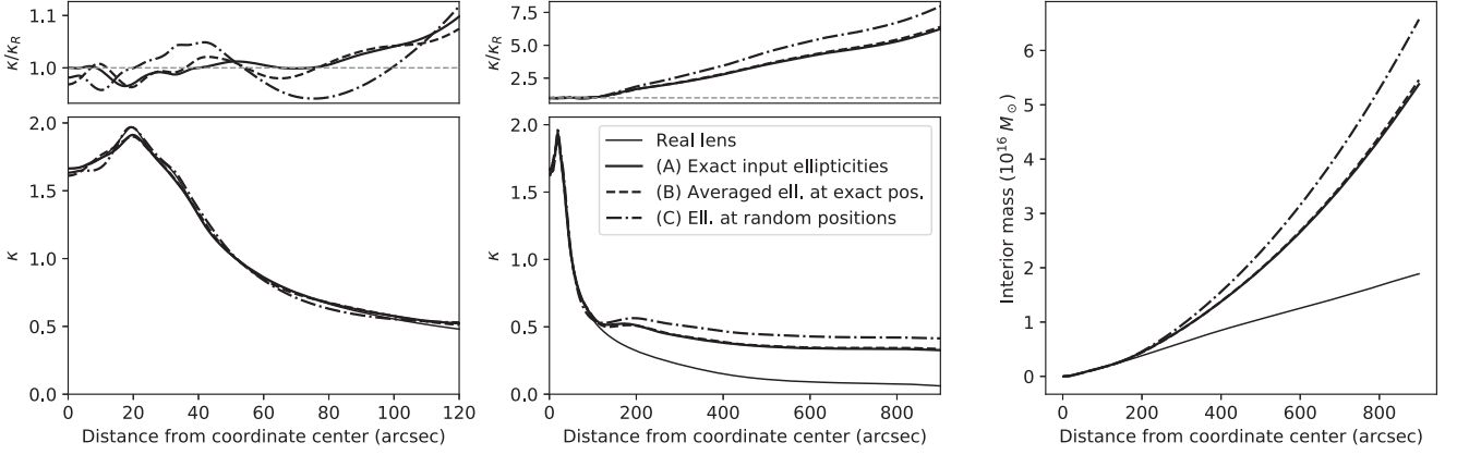
Figure 17. Similar to Fig. 14, but with the mass sheet basis function enabled. The circularly averaged profiles in the strong lensing region (left-hand panel) show a very good correspondence to the true profile in all cases, as can also be seen from the plot of the relative density \kappa/\kappa_R . The profiles for the entire area (centre panel) not only show a considerable mass sheet for scenario (C), where the back-projected images show an improved reconstruction, but also for (A) and (B). The presence of a considerable mass sheet basis function in each case, does not only cause a large ratio of recovered versus true density in the outer regions, but also causes the integrated mass profiles to overestimate the correct enclosed masses in all scenarios (right-hand panel).
