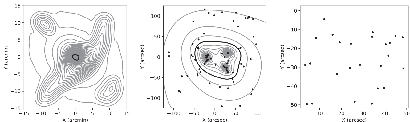
Figure 10. The simulated gravitational lens, at z = 0.4 , used in the weak lensing tests. Left-hand panel: the large-scale mass structure that will be probed by ellipticity measurements with varying degrees of accuracy. The thick line corresponds to \kappa = 1 for a redshift z = 3 . To make the large-scale structure more clearly visible, the contours are separated by a small \Delta\kappa = 0.025 . Centre panel: the strong lensing region of the same mass distribution. The thick line again corresponds to \kappa = 1 , while the contour spacing is now \Delta\kappa = 0.2 . The dots indicate the positions of the 75 point images that are included as constraints. Right-hand panel: the 25 point sources that cause the images from the centre panel.
