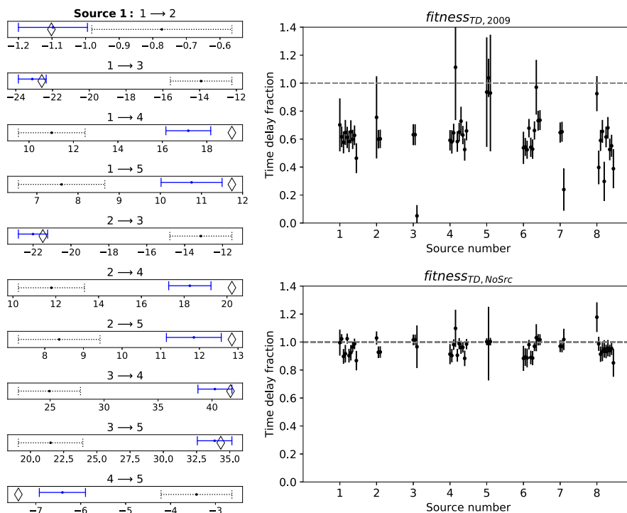
Figure 4. Left-hand panel: this figure compares the predicted time delays to the input ones (diamond symbol) for all image pairs of one particular source, indicated by squares in the centre panel of Fig. 1; the time delays are shown as a number of days. The dotted black line shows the average and standard deviation when the existing fitness_{TD, 2009} is used, whereas the solid blue lines correspond to the new fitness_{TD, NoSrc} . For this system, as well as the ones that are not shown in the figure, the latter fitness measure produces time delay predictions that correspond better to the input time delays. Right-hand panels: instead of showing the time delays themselves for all image pairs, these figures show the fraction of predicted time delay to true time delay for all sources, and for all image pairs per source. The error bars again indicate averages and standard deviations. Clearly, the new fitness measure provides much better correspondence with the true time delays. The fact that fitness_{TD, 2009} produces time delays that are consistently shorter can be largely attributed to the MSD, which would scale time delays by a certain factor. A colour version of this figure is available online.
