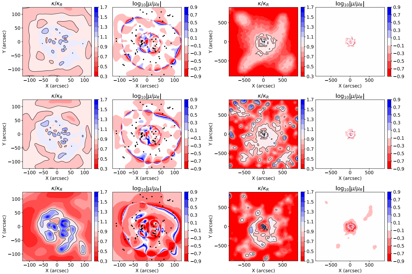
Figure 15. The three rows again correspond to scenarios (A), (B), and (C), and, for the inversions without enabling the mass sheet basis function, show the fractions of recovered densities and magnifications compared to the true ones. The left-hand panels show these fractions for the strong lensing region, the right ones for the weak lensing region. Similar to the circularly averaged profiles, scenarios (A) and (B) show that in the strong lensing region the density traces the true one within 10 per cent (black solid lines) in the central part, while the weak lensing maps reveal a consistently lower reconstructed density. Not only is this underdensity present in (C) as well, but the different steepness in the strong lensing region manifests itself as only a very small part in the 10 per cent range. The strong lensing magnifications confirm what could be seen in the plots of the source plane scales (right-hand panels of Fig. 13: matching scales, and therefore magnifications, for (A) and (B), while the larger source plane scale for (C) corresponds to a lower magnification. For the wider weak lensing regions, the magnifications are more similar, in case (C) suggestive of different MSD scale factors for both strong and weak lensing regions.
