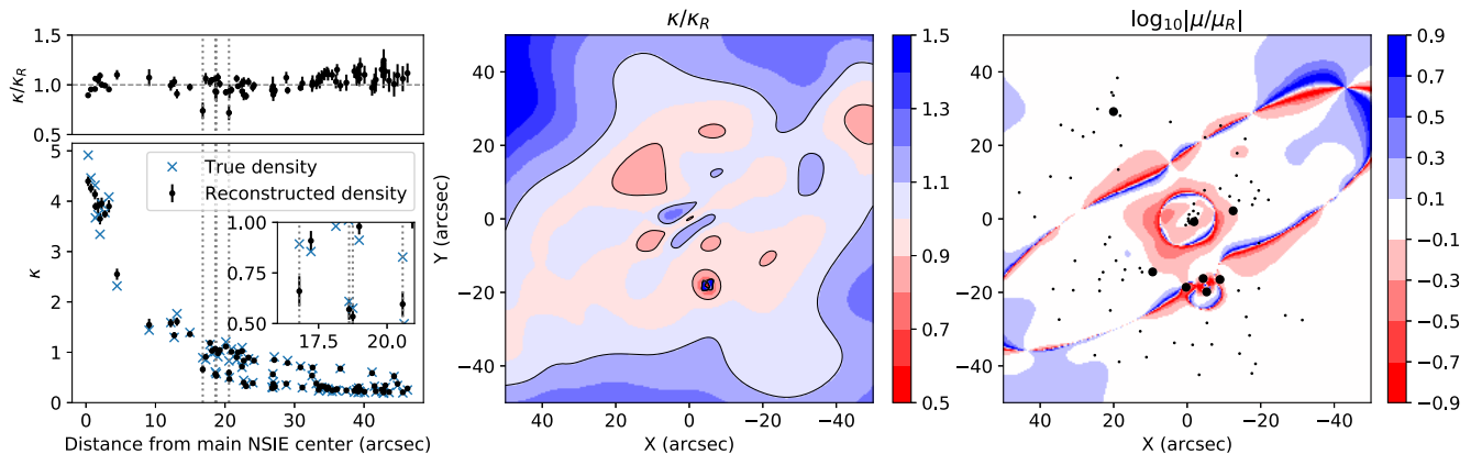
Figure 7. Left-hand panel: using the recovered mass map shown in the right-hand panel of Fig. 5, the densities \kappa at the positions of the images are compared to the densities of the real lens, \kappa_R ; the positions of the quad images are indicated by vertical lines, more clearly discernible in the inset. While there are certainly differences, the overall steepness as well as the density offset appear to be recovered correctly. Centre panel: the relative density, \kappa/\kappa_R , of recovered and true lens models, over the lens plane region; the black line again indicates a change of 10 per cent. This boundary covers a large part of the region, with a notable exception at the position of the quad, indicating that further, more local degeneracies can play a role. Right-hand panel: comparison of the recovered magnification \mu to the one of the real lens model, \mu_R . The correspondence shows much less variation as compared to the example in Fig. 3, undoubtedly due to a less complex mass model needing to be recovered.
