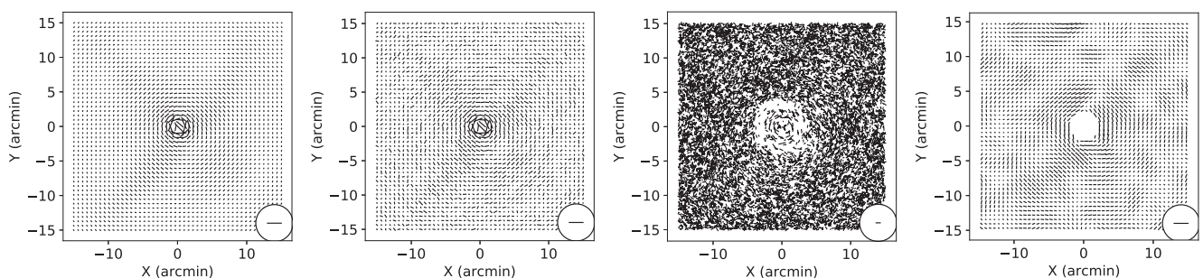
Figure 11. Illustrations of the input ellipticity data used in the three scenarios for the weak lensing tests. First (left most) panel: in scenario (A), the input is the exact ellipticity information calculated from the true model, on a 48 \times 48 grid. Here, the orientation and sizes for z = 1 are shown; the inset shows the size of |\epsilon| = 1 . Second panel: similar, but for scenario (B), where 25 random source ellipticities were transformed at the grid points, and averaged. The result is a more noisy version of the previous ellipticities. Third panel: for scenario (C), 12 000 source ellipticities at different redshifts were transformed. These were binned according to redshift, and on a 48 \times 48 grid the weighted averages were calculated. The last panel shows the result for the bin corresponding to z = 1.5 , one of the inputs in scenario (C). To avoid the less correct weak lensing data affecting the more accurate strong lensing constraints, the central 2 arcmin region was excluded.
