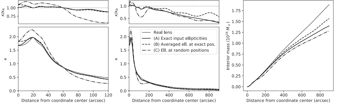
Figure 14. When no mass sheet basis function is used, these profiles are recovered in the weak lensing test. Left-hand panel: the circularly averaged densities in the strong lensing region show a good correspondence for inputs (A) and (B), as can also be seen from looking at the relative density \kappa/\kappa_R , however, the steepness and density offset are quite different when the input from scenario (C) is used. Centre panel: the circularly averaged densities over the entire weak lensing area. Interestingly, even though the strong lensing region is recovered incorrectly for scenario (C), beyond \sim 200 arcsec the profile matches the other ones quite well visually, yet upon inspection of the \kappa/\kappa_R ratio it becomes clear that actually all reconstructions underestimate the real density. Right-hand panel: the integrated mass profiles as well show that in each one of the reconstructions the total mass is underestimated.
