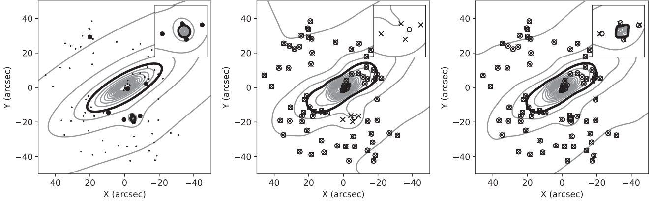
Figure 5. Left-hand panel: the mass distribution used to study the situation where small-scale substructure causes an extra quad to appear. Both large-scale distribution and small perturbation are modelled using NSIE lenses, placed at z = 0.4 . The contours indicate lines of equal convergence \kappa , calculated for a redshift of z = 1.5 , which is the redshift of the multiple image system containing the quad (filled circles); the inset shows this region in more detail. The thick solid line indicates \kappa = 1 , the spacing between contours corresponds to \Delta\kappa = 0.25 . Small points indicate the other point images. Centre panel: the default subdivision procedure leads to this reconstruction, an average of 20 individual reconstructions. The input point images are shown as crosses, the corresponding images predicted by the model as open circles. As shown in the inset, the quad images cannot be reproduced, as the required density perturbation is not recovered. Right-hand panel: similar to the centre panel, but this time extra basis functions were used to allow for a smaller resolution in between the quad images (see text). This time, the quad can indeed be reproduced.
