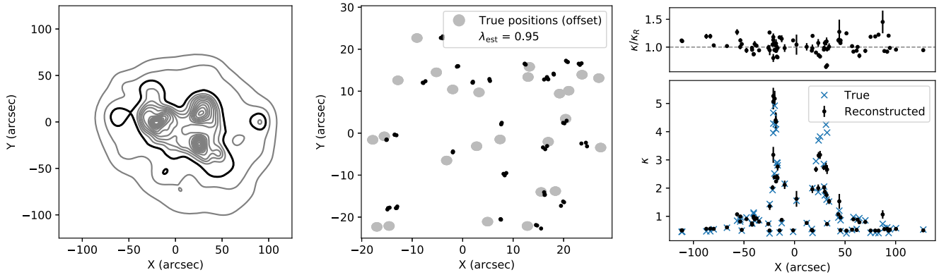
Figure 12. Using only the strong lensing constraints for the simulated lens of Fig. 10, these results are obtained. Left-hand panel: the average mass map of 20 individual runs, where the mass sheet basis function was included. The general features of the true mass distribution could be recovered. Centre panel: comparing the true source positions to the back-projected images shows that overall, the scales correspond well, although there is slight overfocusing. The diameter of the filled grey circles is 2 arcsec. Right-hand panel: a comparison of the true and recovered densities at the image positions, of which the x -coordinate is used on the horizontal axis, shows no obvious differences in density offset or steepness.
