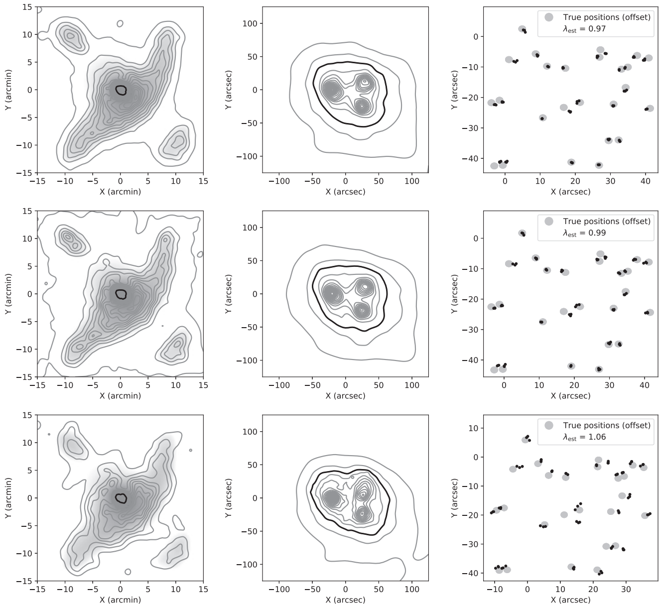
Figure 16. Similar to Fig. 13, but with the mass sheet basis function enabled. In all cases the structure shape in the weak lensing region is recovered (left-hand panels), albeit with different levels of accuracy and somewhat different density offsets. The recovered strong lensing mass (centre panels) is very similar in each case, and the back-projected images overlap well (right-hand panels). The recovered source plane scales match the true ones in all three cases, as can be seen from their \lambda_{\text{est}} estimates, indicating that the MSD scale factor is recovered well in the strong lensing region.
