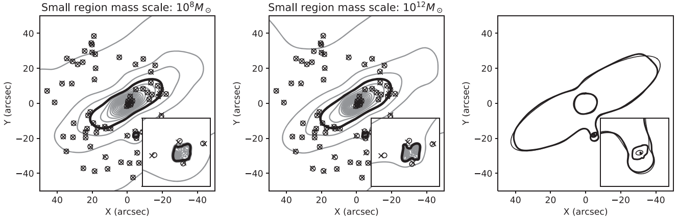
Figure 8. The first two panels show results similar to the right-hand panel of Fig. 5, but for different settings of the mass scale in the region of the small density peak (see text). The right-hand panel shows the critical lines at the redshift z = 1.5 of the source, for both the reconstruction from the right-hand panel of Fig. 5, and the true lens.
