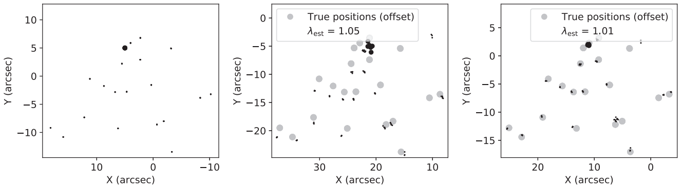
Figure 6. Left-hand panel: the 20 true source positions that generate the multiple image systems shown in the left-hand panel of Fig. 5. Here too, the source responsible for the quad is shown as a filled circle. Centre panel: the back-projected images using the reconstruction in the centre panel of the same figure, compared to the true source positions; the diameter of the grey circles is 1 arcsec. Similar to a previous example, the true source positions are shown with an offset, to be able to compare true and recovered source plane scales. While the overall scale is recovered well, as are most sources, especially the images of the quad system do not coincide satisfactorily. Right-hand panel: same, but using the reconstruction of the right-hand panel of Fig. 5. The agreement of the source plane scales is even more similar, but especially noticeable is the fact that the points of the quad system now overlap to a much better degree.
