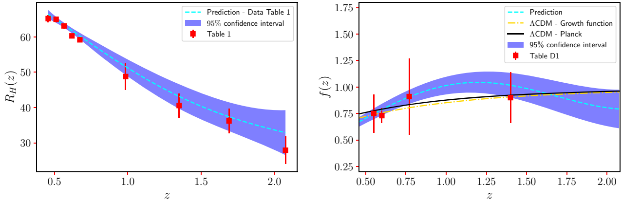
Figure 2. Left-hand panel: Reconstruction of the homogeneity scale function R_H(z) using Gaussian Process (dashed line) and the R_H measurements (red squares) presented in Table 1 (see the text for details about the data set); the shadow represents the 95 per cent CL. Right-hand panel: Derivation of the growth rate of structures f^{R_H}(z) (dashed line) using the reconstructed function R_H(z) , shown in the left-hand panel plot, and the equation (26), where the shadow represents the 95 per cent CL. The solid line represents the expression expected in the \Lambda CDM model, f^{\Lambda\text{CDM}}(z) , obtained from equation (6) with \Omega_m^{\text{Planck}} = 0.315 ; instead, the dot-dashed line shows the expected growth rate using equation (6) but with \Omega_m = 0.270_{-0.073}^{+0.079} , a value obtained from the best-fitting analyses of the f(z) data as shown in Fig. 4 (the red squares are the data listed in Table D1). Comparing the f^{R_H}(z) (dashed line) and the best-fitting f(z) (dot-dashed line) functions we found an agreement of <2\sigma (considering the corresponding uncertainties, not shown in the figure to avoid excess of information).
