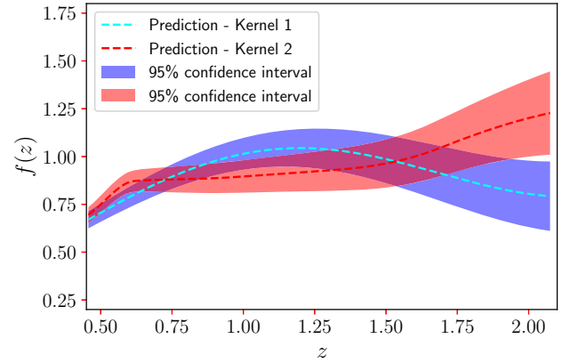
Figure C1. The reconstruction of the growth rate of structures f^{RH}(z) using two different kernels, namely, kernel 1 (the SE kernel) and kernel 2 (the Matérn kernel).
