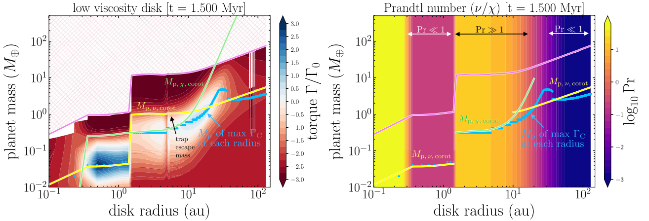
Figure 11. The planet mass of maximum outward torque in the limits of Pr \ll 1 and Pr \gg 1 . [Low viscosity, high-mass disc]. Here, we illustrate how well our two analytic approximations for the planet mass of maximum outward torque agree with the numerically calculated values from our torque maps. Left-hand panel: Atop the total torque map of the high-mass, low viscosity disc, we show the numerically calculated planet mass of maximum outward torque at each radius (blue dots), the viscous M_{p, \nu, \text{corot}} based on p_\nu (yellow line), and the thermal M_{p, \chi, \text{corot}} based on p_\chi (light green line). Right-hand panel: Same as the left-hand panel, but overlaid on a map of Prandtl number ( Pr = Pr(r) = \nu/\chi , see right-hand panel of online Fig. C1). The M_{p, \nu, \text{corot}} curve predicts what planet masses are required for outward migration in regions where Pr \ll 1 , and M_{p, \chi, \text{corot}} does the same where Pr \gg 1 . When each curve is not describing M_p of maximum \Gamma_C , it is delineating the boundary to inward migration (e.g. M_{p, \nu, \text{corot}} describes the water iceline escape mass). See left-hand panel of online Fig. C1 for the same curves overlaid on purely the corotation torque map.
