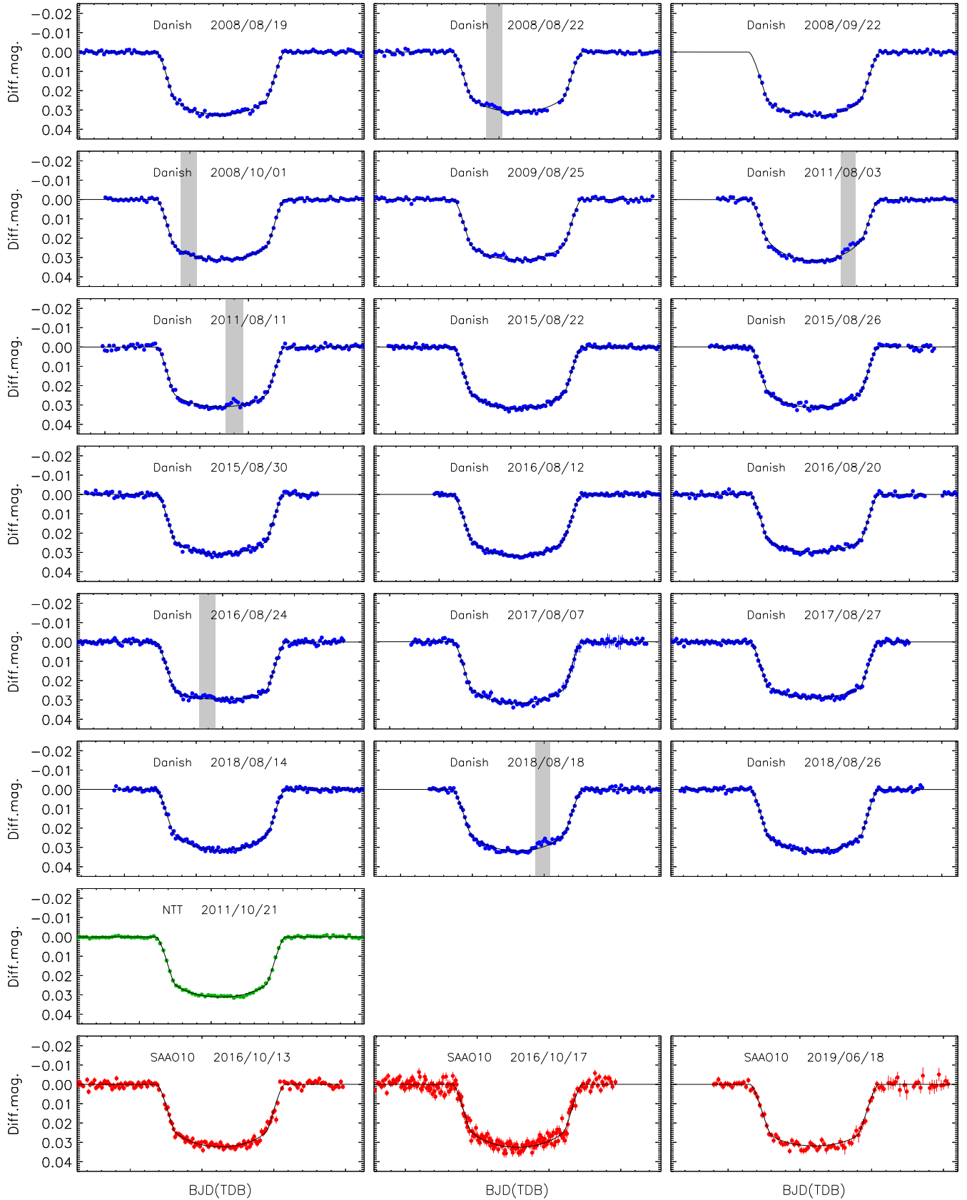
Figure 1. All new photometric data presented in this work. In each case the x -axis shows 0.2 d centred on the time of minimum measured for that transit. The telescope and date are labelled on each panel. Star-spot crossing events are visible during totality in six of the light curves, and are indicated by the grey boxes. The JKTEBOP best fits are shown using black lines.
