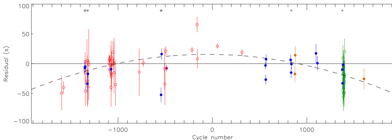
Figure 2. Plot of the residuals of the timings of mid-transit versus a linear ephemeris. The results from this work are shown with filled circles: blue for the Danish telescope, orange for the SAAO 1.0 m, and purple for the NTT. Published results are shown using open circles: red for the literature data collected by B19 and green for the TESS timings from B19. The dotted line shows the difference between the best-fitting linear and quadratic ephemerides. Grey asterisks have been placed near the top of the figure to indicate transit times measured from a light curve with a spot crossing event.
