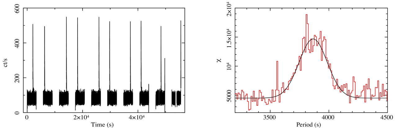
Figure 5. Light curve of the 10 type-I bursts observed by NuSTAR in 2015 during the intermediate state ( left ) and folding of the light curve, fitted with a Gaussian model ( right ). The zero in the light curve corresponds to the Modified Julian Date (MJD) 57113.6798.
