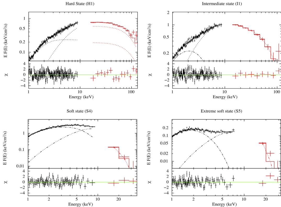
Figure 2. XRT (black) and BAT (red) spectra of Obs. labelled as: H1 (top, left), I1 (top, right), S4 (bottom, left), and S5 (bottom, right) and relative residuals. In H1, we used the model COMP TB+COMP TB, in I1 we used DISKBB+COMP TB, while a BBODY+DISKBB model was employed for both S4 and S5. We adopted different linestyles to distinguish between the different components, in particular we used dot for COMP TB, dot-dashed for DISKBB and dash-dot-dot-dotted for BBODY.
