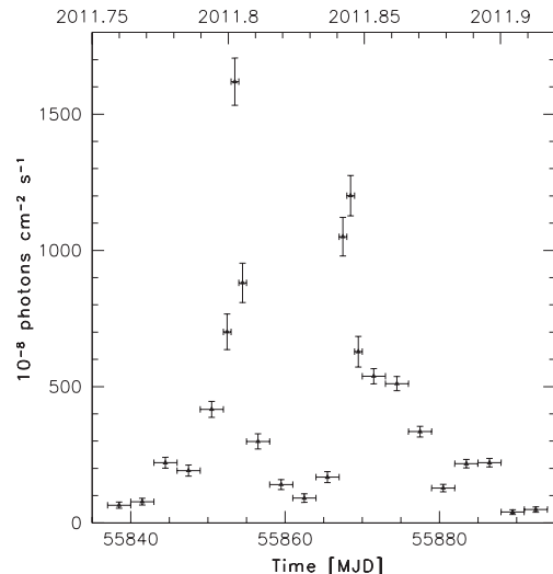
Figure 3. Integrated flux ( E > 100 MeV) light curve of PKS 1510–089 obtained from 2011 October 3 to November 28 (MJD 558 37–558 93) with either 1-d (close to the peak) or 3-d time bins.
