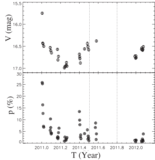
Figure 11. Optical V-band light curve ( top ) and polarization percentage ( bottom ) of PKS 1510–089 between 2011 January and 2012 January. The vertical lines indicate the time of the \gamma -ray flares.
