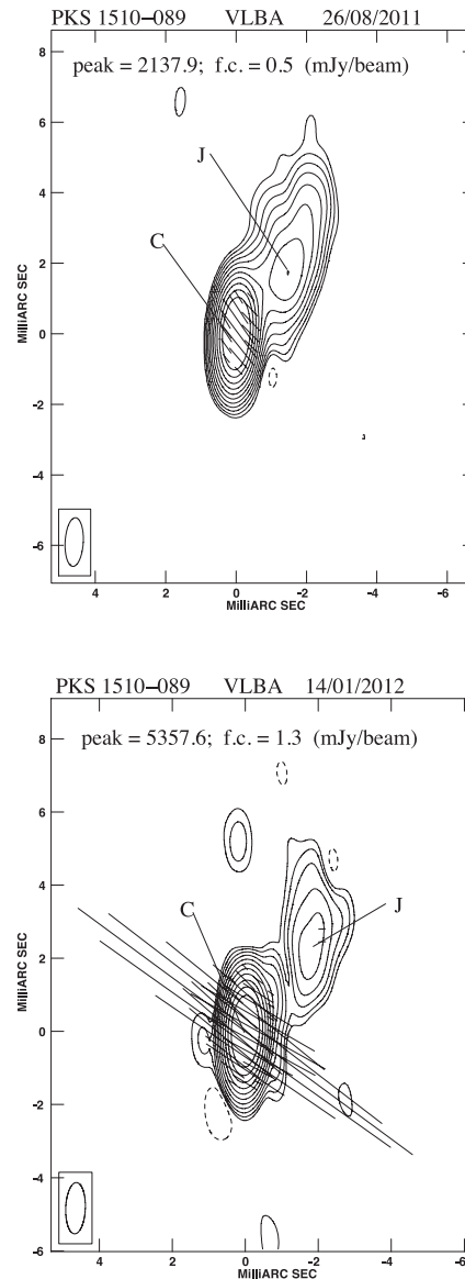
Figure 8. 15-GHz VLBA images of PKS 1510–089 relative to 2011 August ( upper panel ) and 2012 January ( bottom panel ). On each image, we provide the telescope array and the observing date; the peak flux density is in mJy/beam and the first contour ( f.c. ) intensity is in mJy/beam, which corresponds to three times the off-source noise level. Contour levels increase by a factor of 2. The restoring beam is plotted in the bottom-left corner. For the data sets with polarization information, the vectors superimposed on the I contours show the position angle of the E vector, where 1 mas length corresponds to 14.3 mJy/beam.
