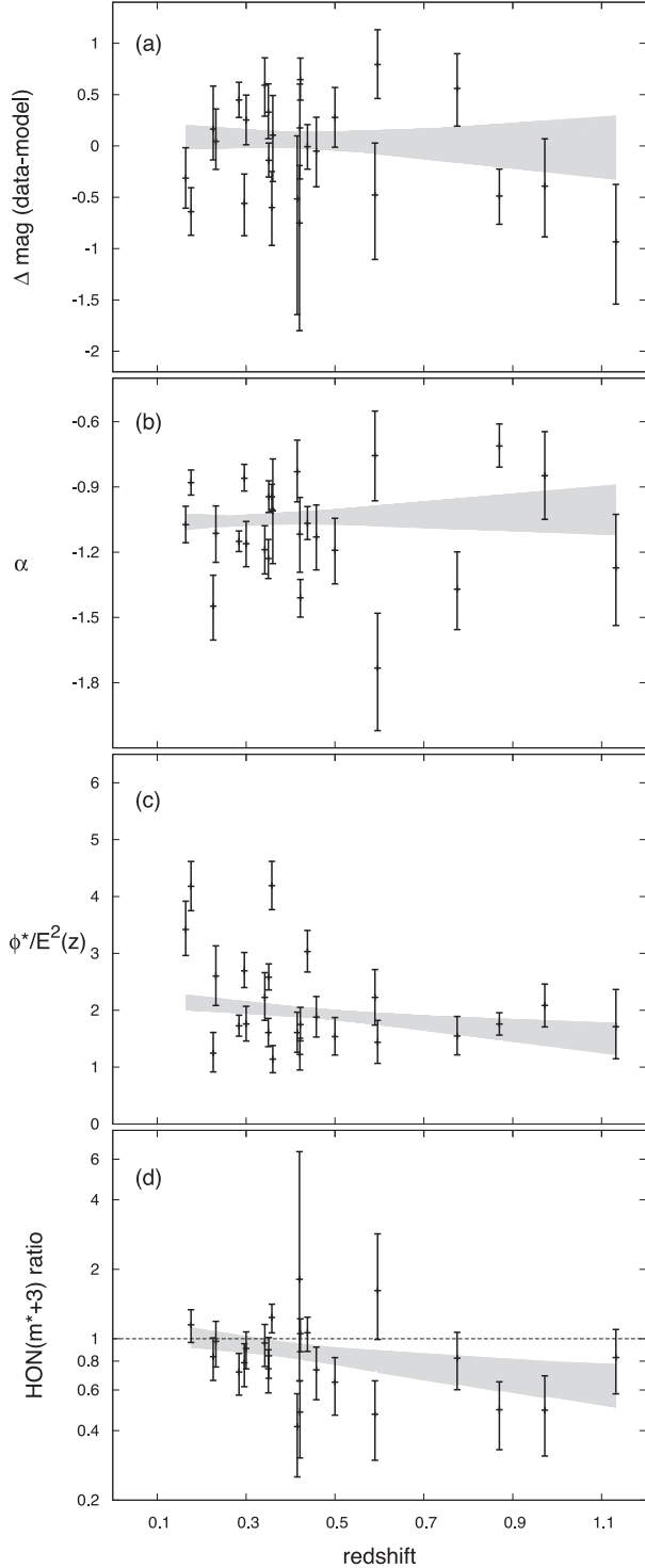
Figure 5. LF parameter evolution with redshift. As noted before, the LFs are extracted using the band redward of the 4000 Å break. We fit a line in each case, marking the allowed 1\sigma region. Panel (a): there is no significant evolution in \Delta\text{mag} = (m_{\text{model}}^* - m^*) , indicating the CSP model provides a good description of cluster galaxies over this redshift range. Panel (b): evolution of \alpha is suggested by the data with best-fitting line having intercept -1.05^{+0.05}_{-0.05} and slope -0.04^{+0.14}_{-0.14} . Panel (c): \phi^*/E^2(z) extracted when fixed m^* is consistent with no evolution at 2.38\sigma level. Panel (d): ratio of HON from this work and the redshift-independent L04 prediction. Slope and intercept are found to be -0.80^{+0.38}_{-0.38} and 0.06^{+0.06}_{-0.05} at 1\sigma , respectively, which indicate a mild evolution where z = 1 clusters have typically 30 per cent fewer galaxies than their low-redshift counterparts of the same mass.
